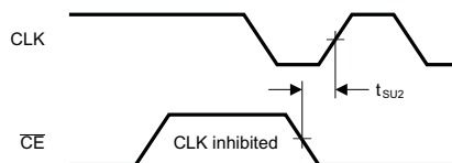
Figure 7. Serial – Shift Clock Inhibit Mode
