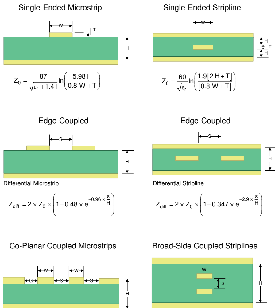
Figure 8-4. Controlled-Impedance Transmission Lines
