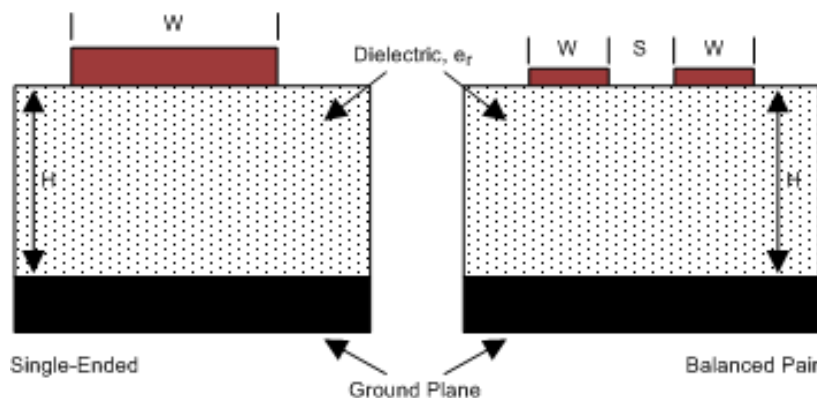
Figure 10-1. Microstrip Topology
