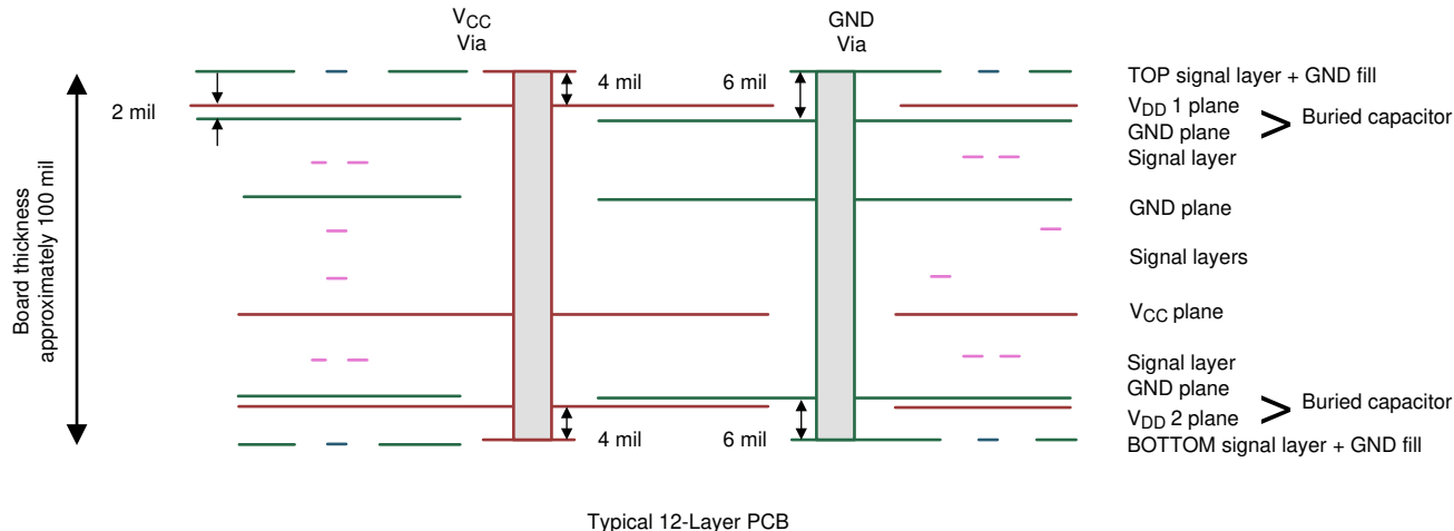
Figure 10-6. Low Inductance, High-Capacitance Power Connection
