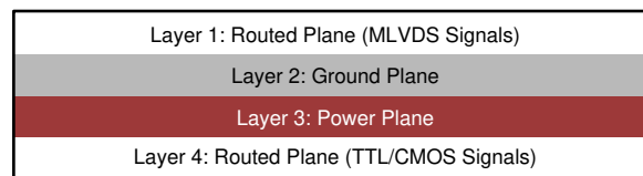
Figure 10-3. Four-Layer PCB Board
