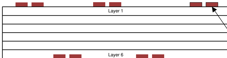
Figure 10-7. Staggered Trace Layout
