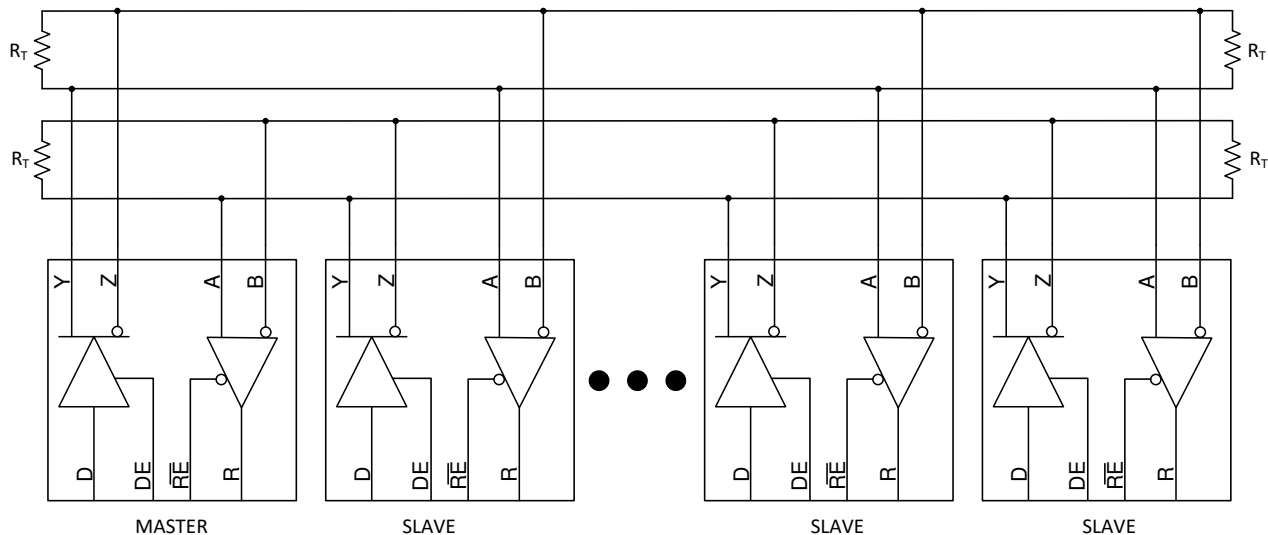
Figure 8-1. Multipoint Configuration
