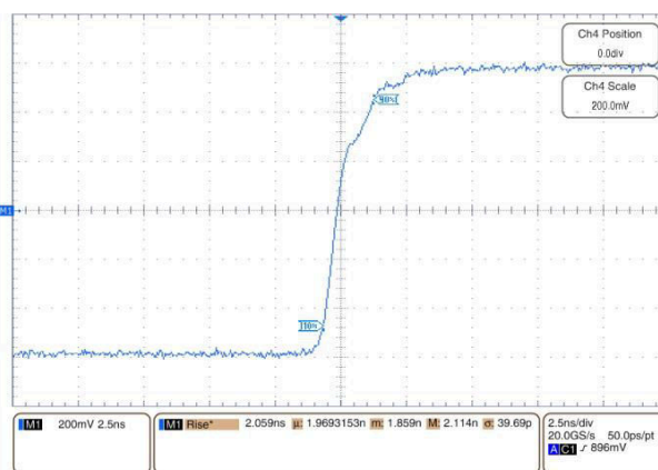
Figure 8-6. Driver Rise Time
