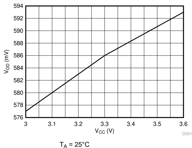
Figure 5-1. Differential Output Voltage vs Supply Voltage
