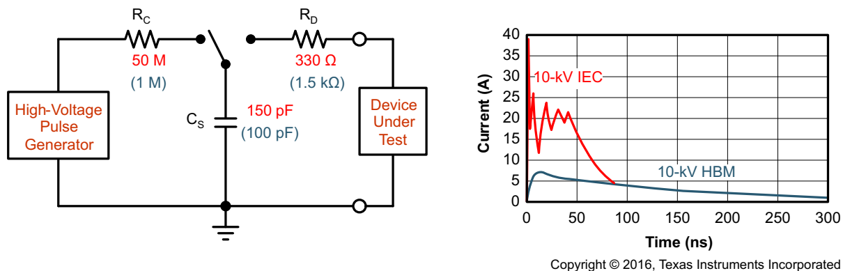
Figure 7-1. HBM and IEC-ESD Models and Currents in Comparison (HBM Values in Parenthesis)
