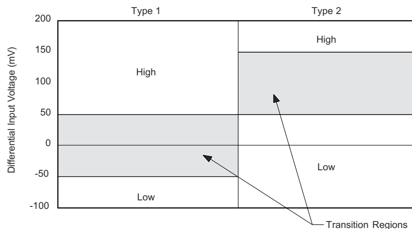
Figure 8-3. Expanded Graph of Receiver Differential Input Voltage Showing Transition Region
