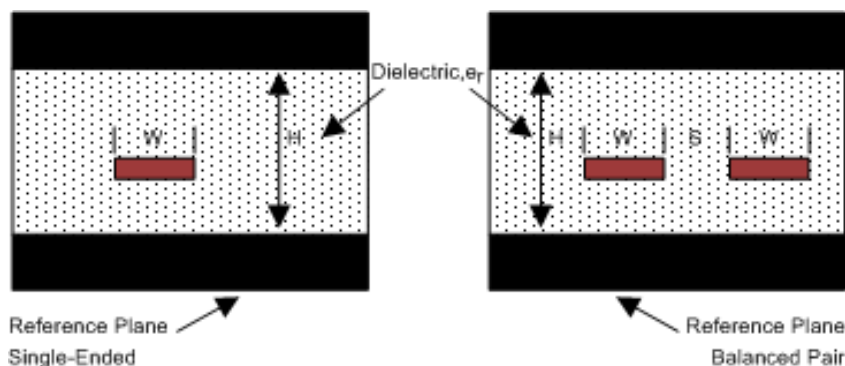
Figure 10-2. Stripline Topology
