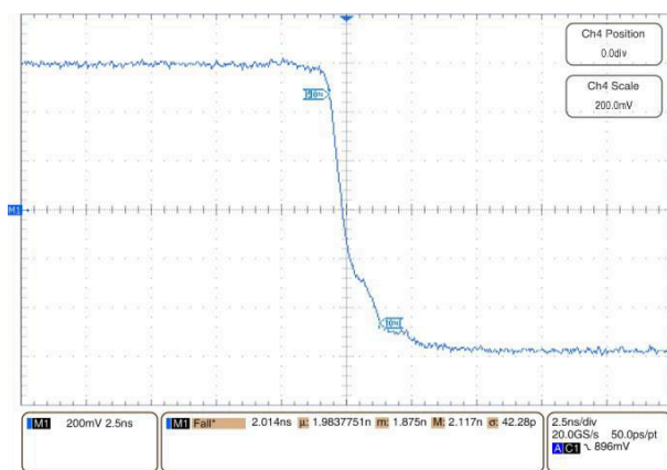
Figure 8-5. Driver Fall Time
