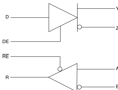
Simplified Schematic, SN65MLVD203B
