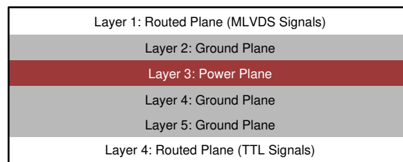
Figure 10-4. Six-Layer PCB Board
