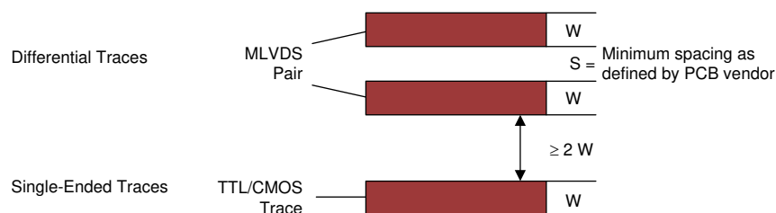
Figure 10-5. 3-W Rule for Single-Ended and Differential Traces (Top View)
