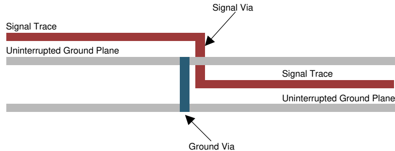
Figure 10-8. Ground Via Location (Side View)
