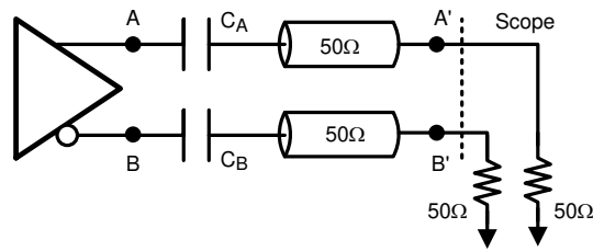
Figure 1. Serializer Test Circuit
