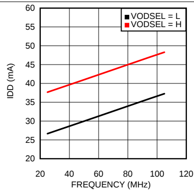
图 13. Typ Current Draw — Single In/Single Out Mode — PRBS-7 Data Pattern
