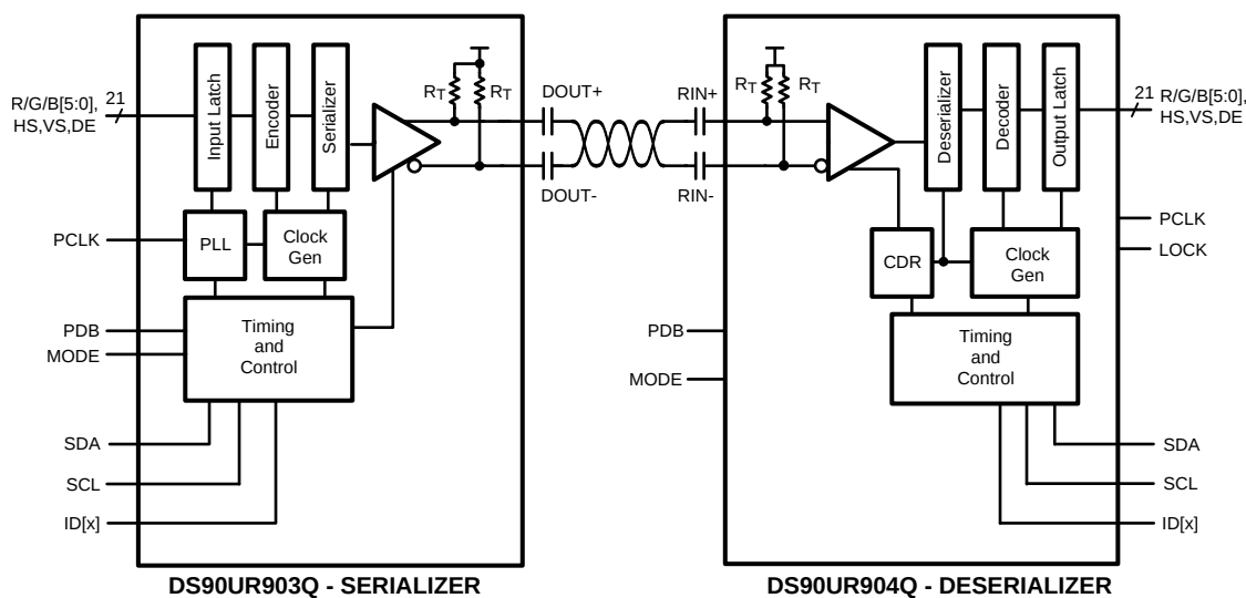
Figure 21. Block Diagram
