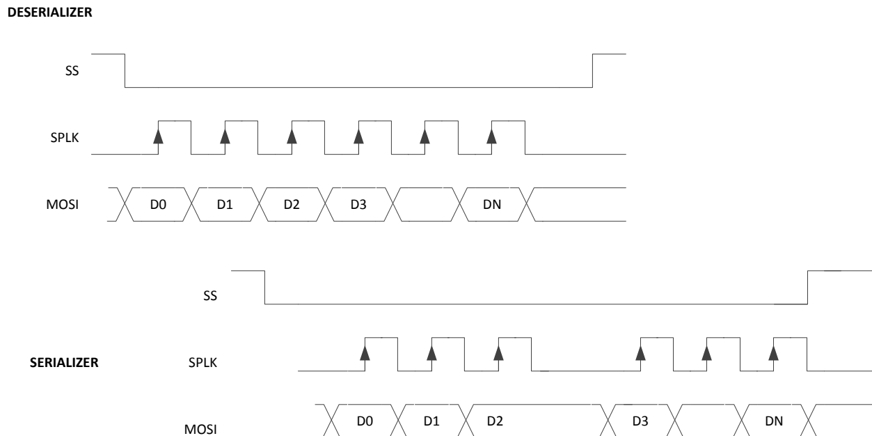
图 11. Reverse Channel SPI Write
