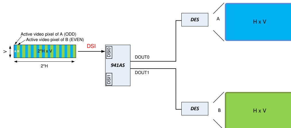
图 30. Alternate Pixel Splitting
