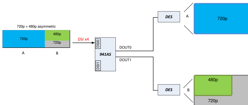
图 32. Asymmetric Splitting With Cropping
