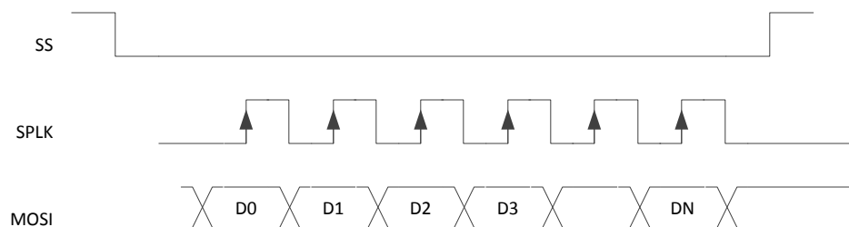
图 9. Forward Channel SPI Write
