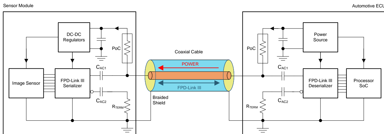
图 39. Power-Over-Coax (PoC) System Diagram
