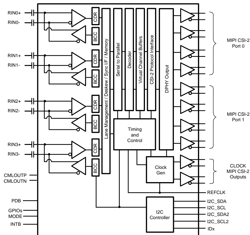
图 13. Functional Block Diagram
