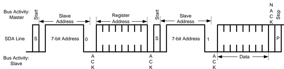
图 36. Serial Control Bus — READ
