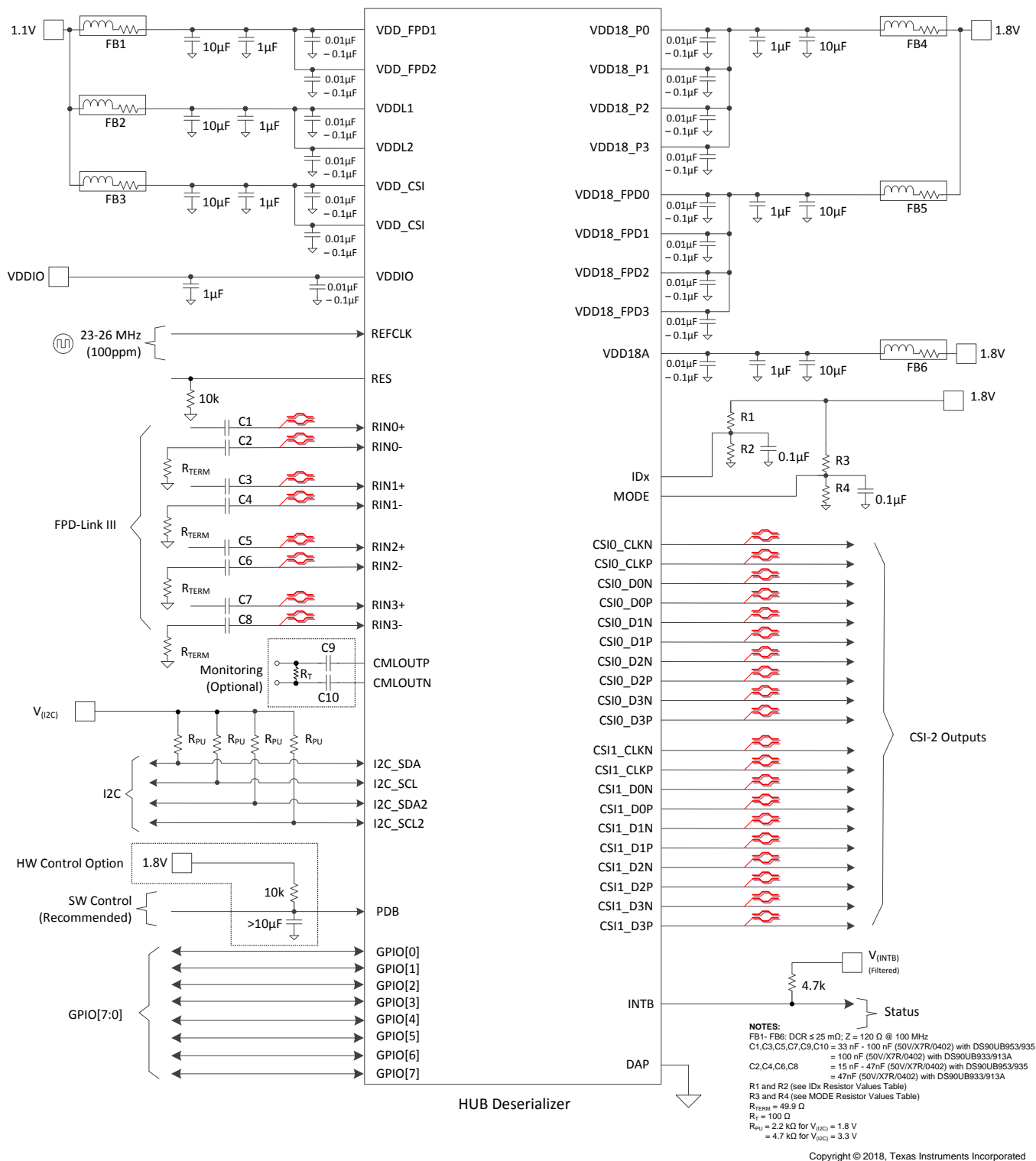
图 42. Typical Connection Diagram (Coaxial)
