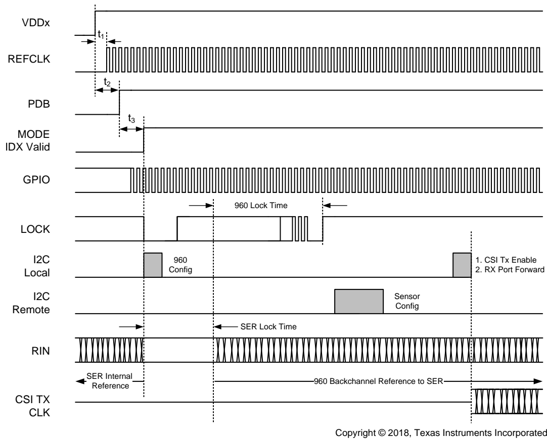
图 57. Power-Up Sequencing with Synchronous Clocking Mode
