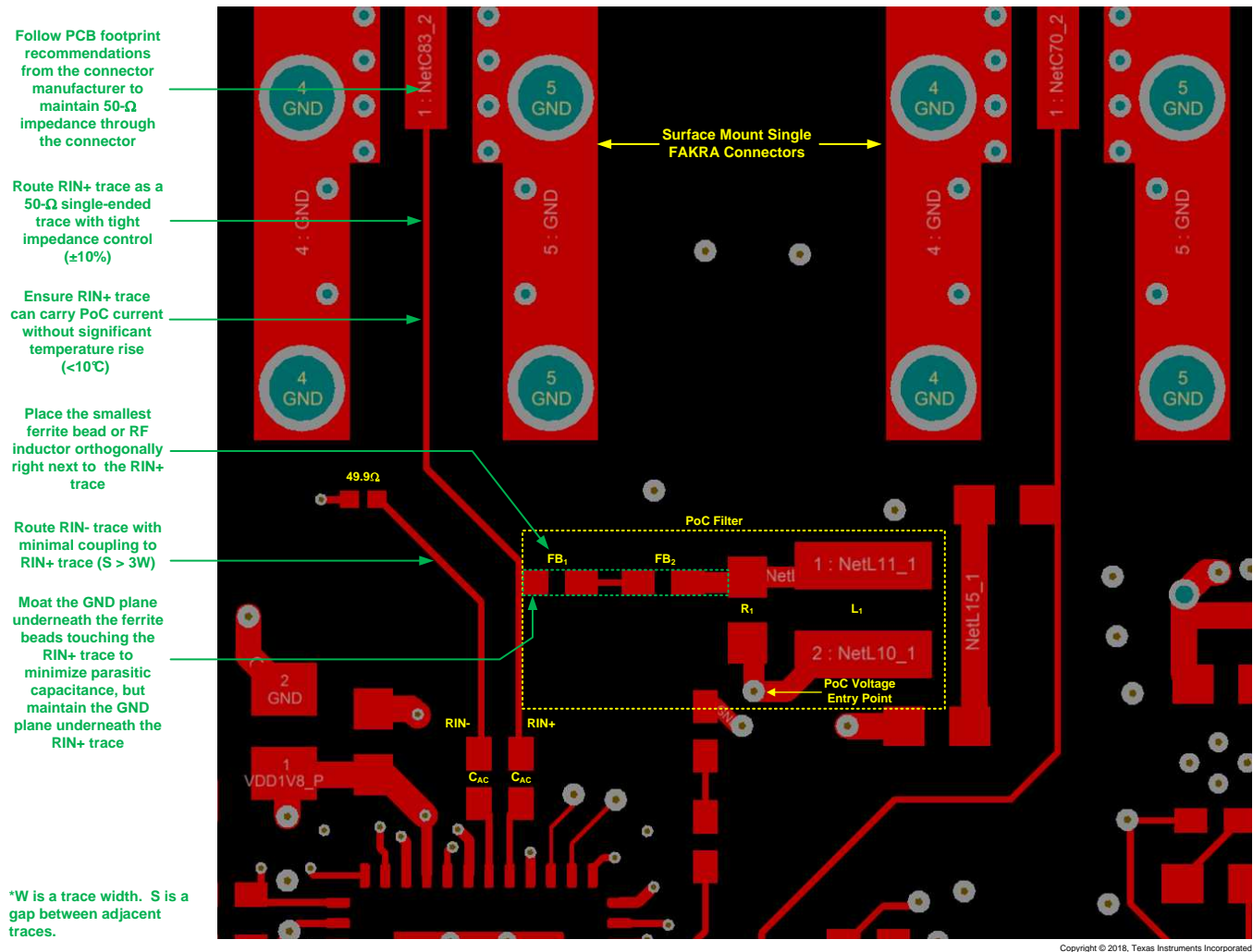
图 60. Example Routing of FPD-Link III Traces to a Single Mini-Fakra Connector and PoC Components
