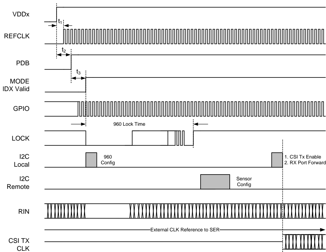
图 58. Power-Up Sequencing with Non-synchronous Clocking Mode
