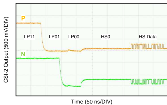
图 48. CSI-2 Start of Transmission (SoT)
