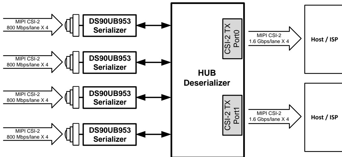
图 50. Four DS90UB953-Q1 Sensor Data Onto CSI-2 Over 2 Ports
