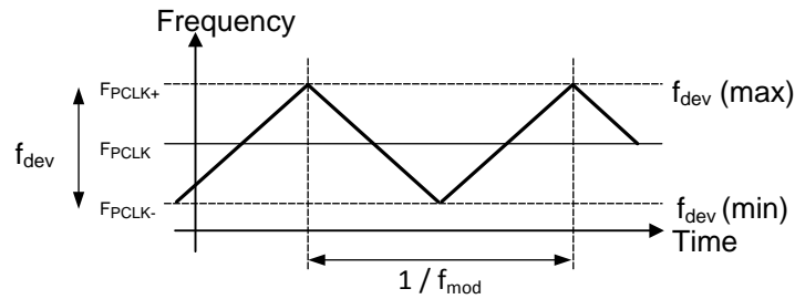
图 9. Spread Spectrum Clock Output Profile
