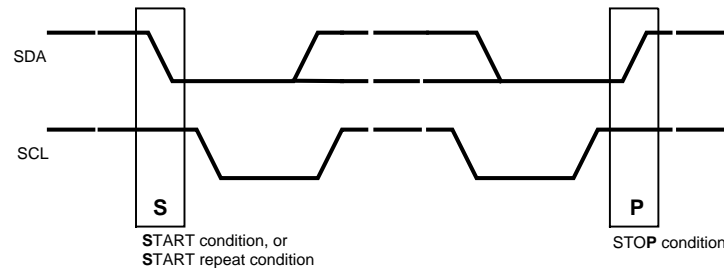
图 18. START and STOP Conditions
