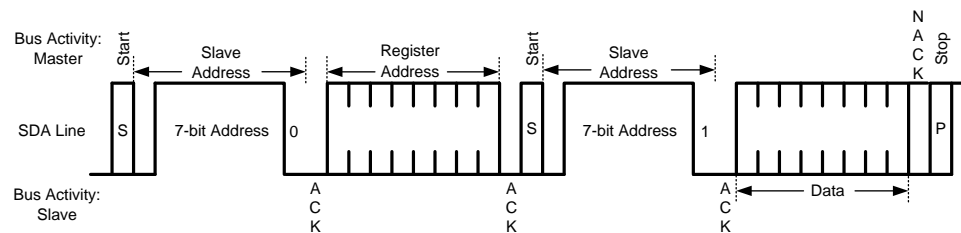
图 19. Serial Control Bus — READ
