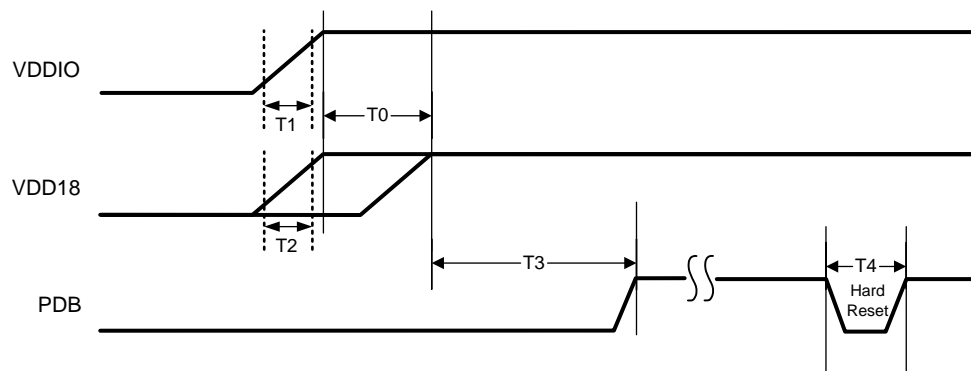
图 32. Power-Up Sequencing
