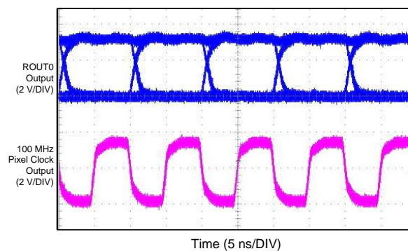
图 11. ROUT0 Data Sampled by 100-MHz PCLK RRFB (0x3B[0]) = 1
