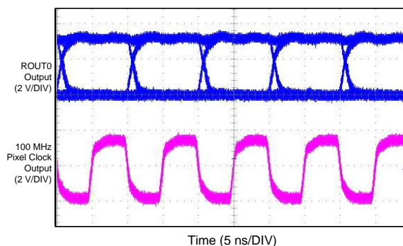
图 29. ROUT0 Data Sampled by 100-MHz PCLK RRFB (0x3B[0]) = 1
