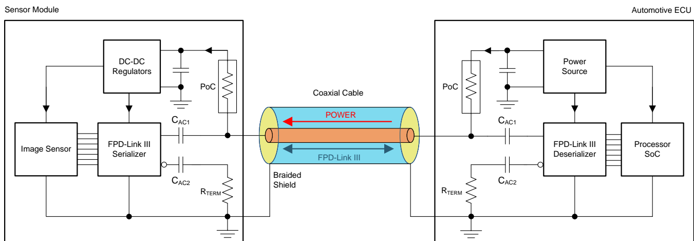
图 22. Power Over Coax (PoC) System Diagram
