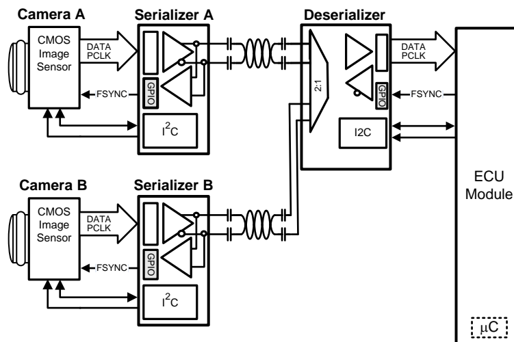
图 12. Using the Multiplexer on the Deserializer to Enable a Two-Camera System
