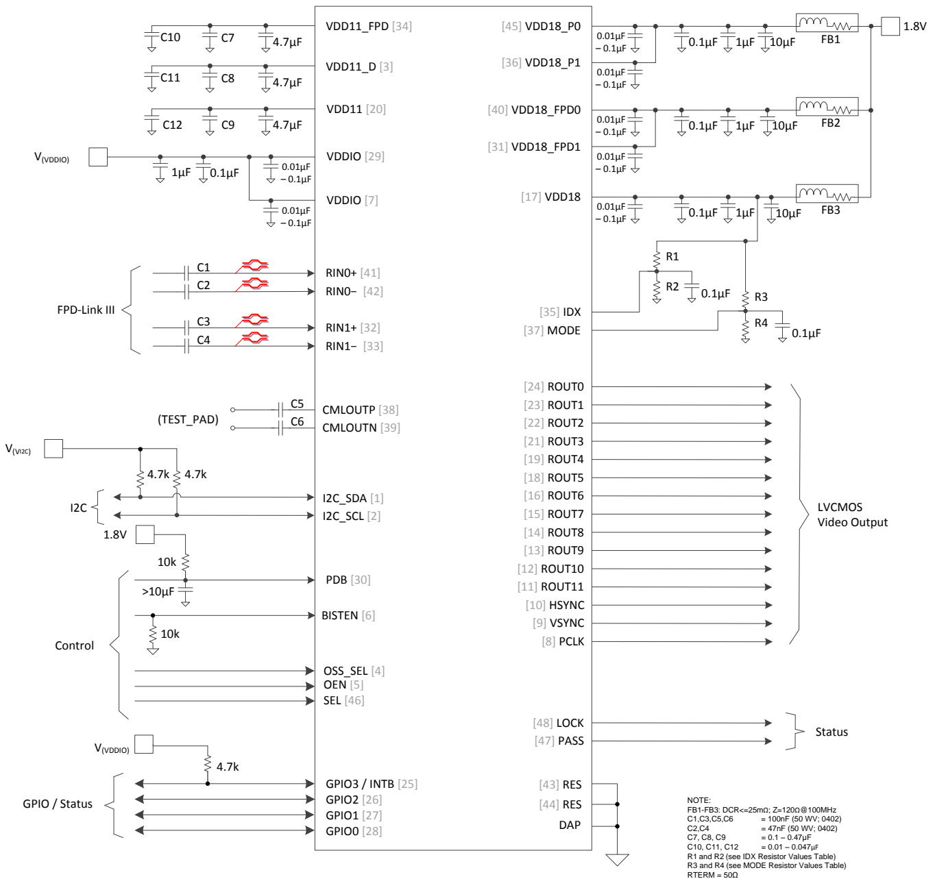
图 25. Typical Connection Diagram STP
