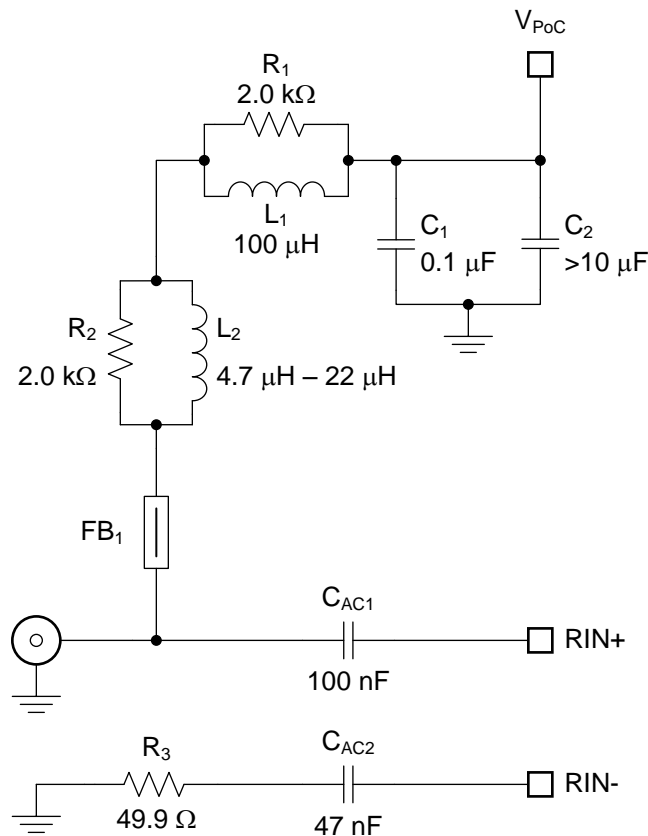
图 23. Typical PoC Network for a 2G FPD-Link III
