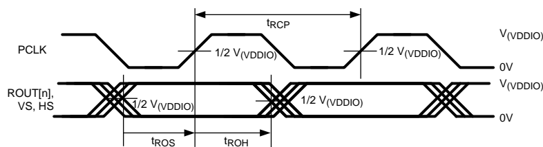
图 7. Deserializer Output Setup/Hold Times
