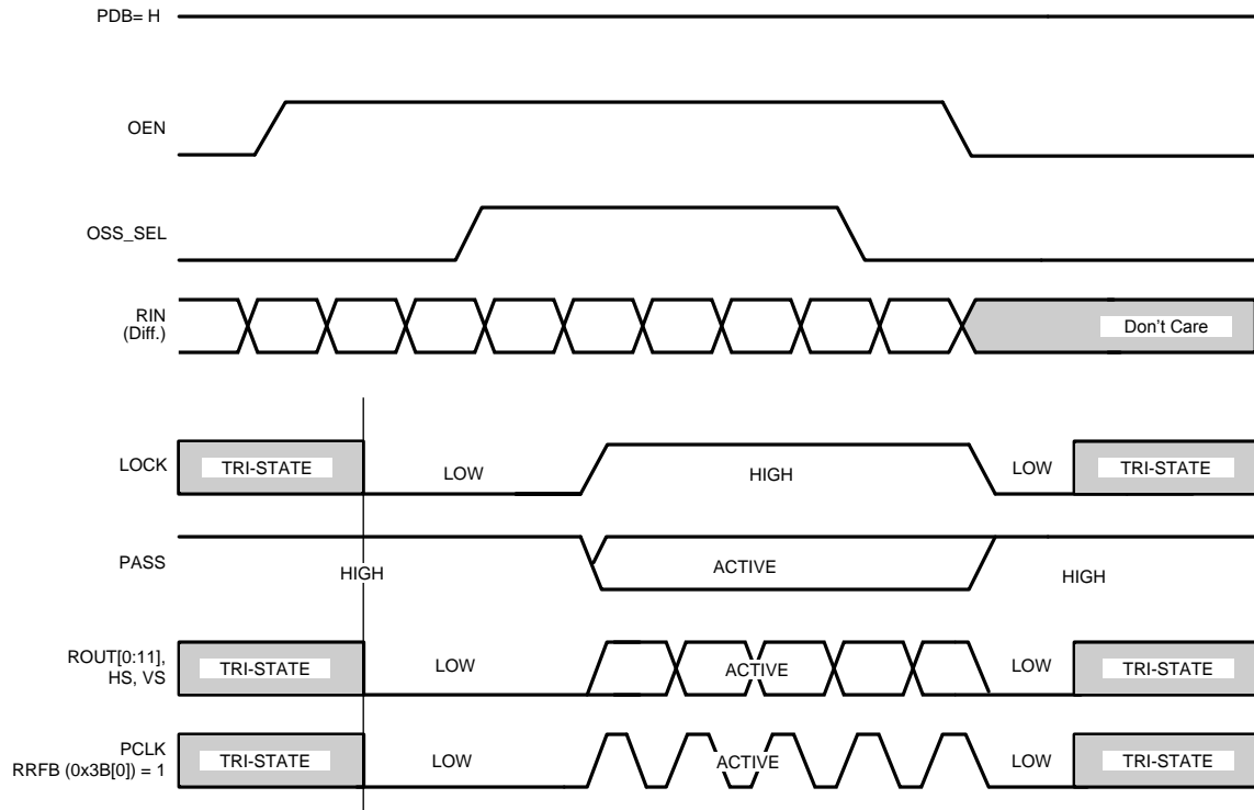
图 8. Output State (Setup and Hold) Times
