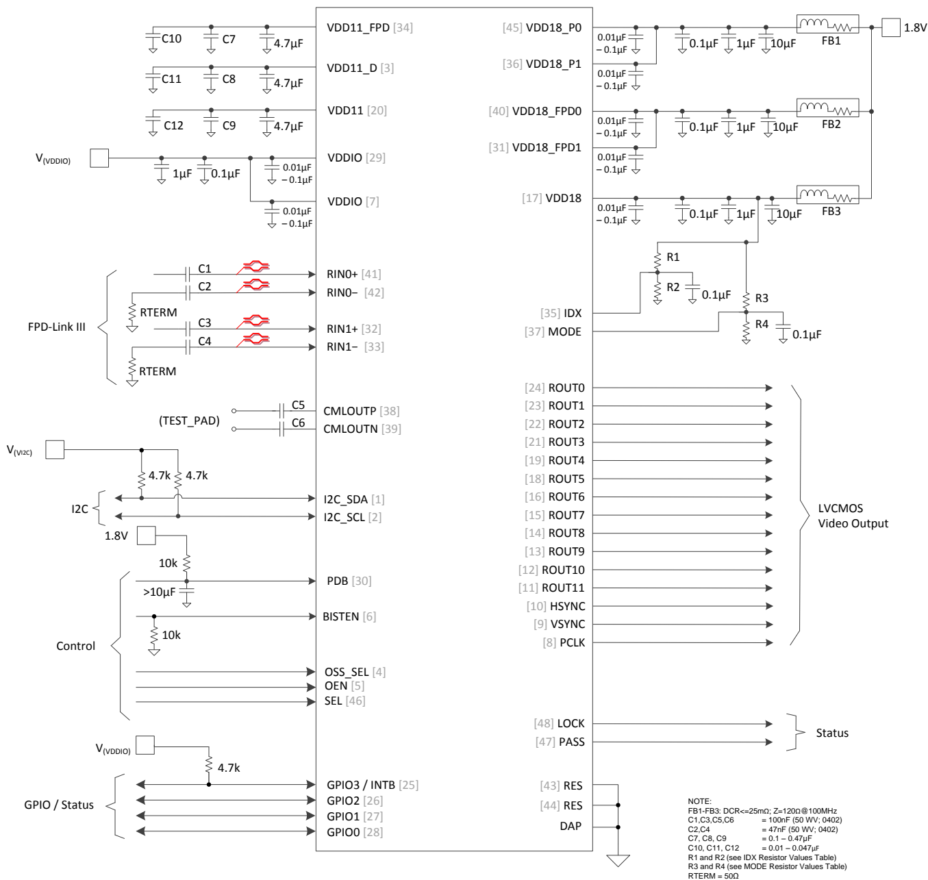
图 24. Typical Connection Diagram Coaxial
