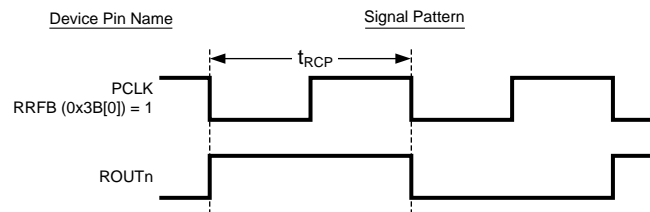
图 5. SSO Test Pattern for Power Consumption
