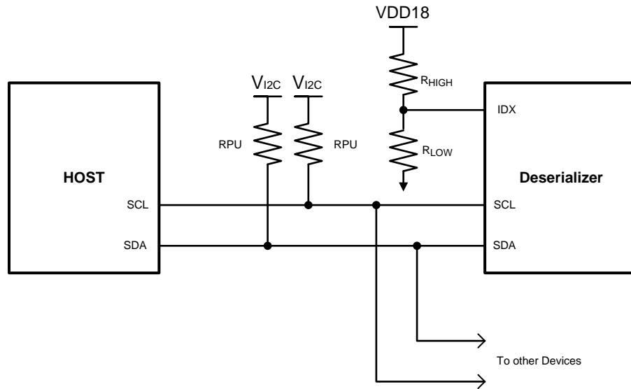
图 17. Serial Control Bus Connection
