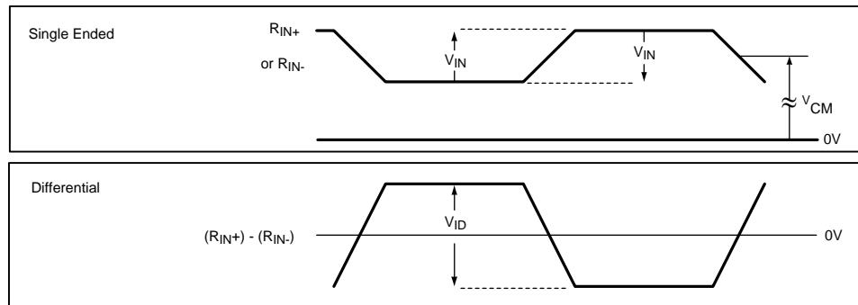
图 2. FPD-Link III Receiver V_{\text{ID}} , V_{\text{IN}} , V_{\text{CM}}
