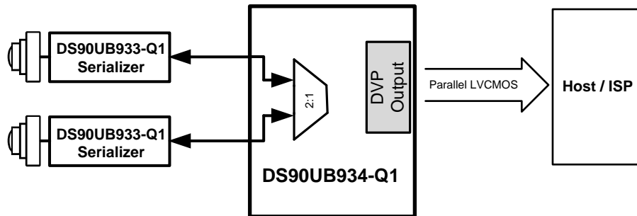
图 31. Two DS90UB933-Q1 Camera Data to 2 Rx Ports
