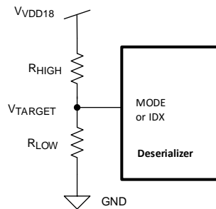
图 13. Strap Pin Connection Diagram
