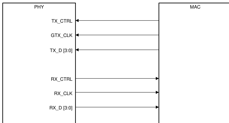
Figure 7-2. RGMII Connections
