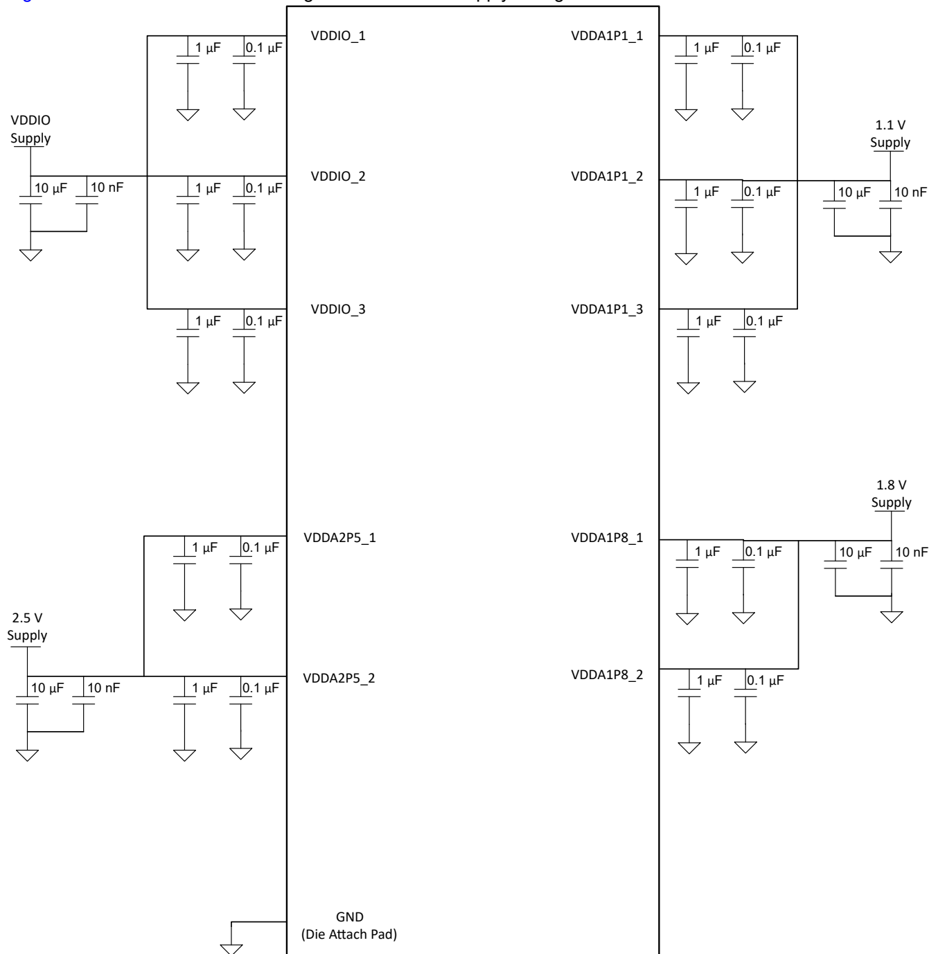
Figure 9-3. Three-Supply Configuration
