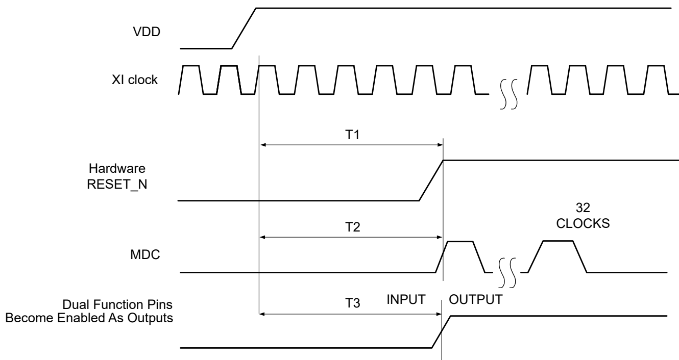
Figure 6-1. Power-Up Timing
