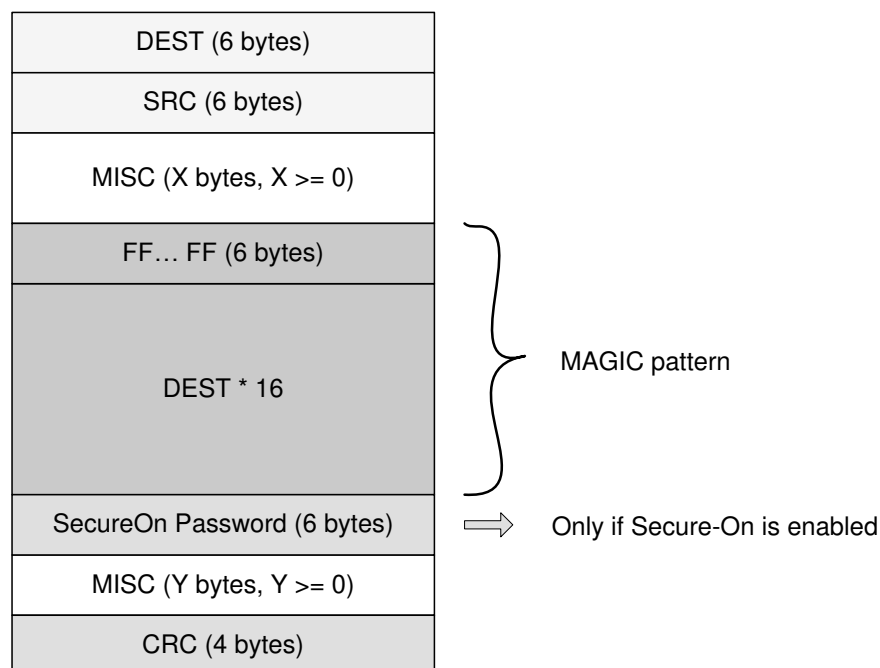
Figure 7-4. Magic Packet Structure
