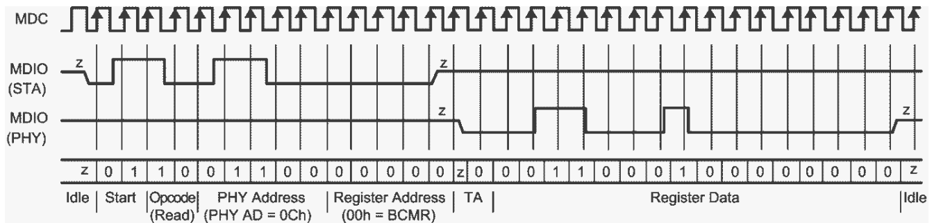
Figure 7-10. Typical MDC/MDIO Read Operation
