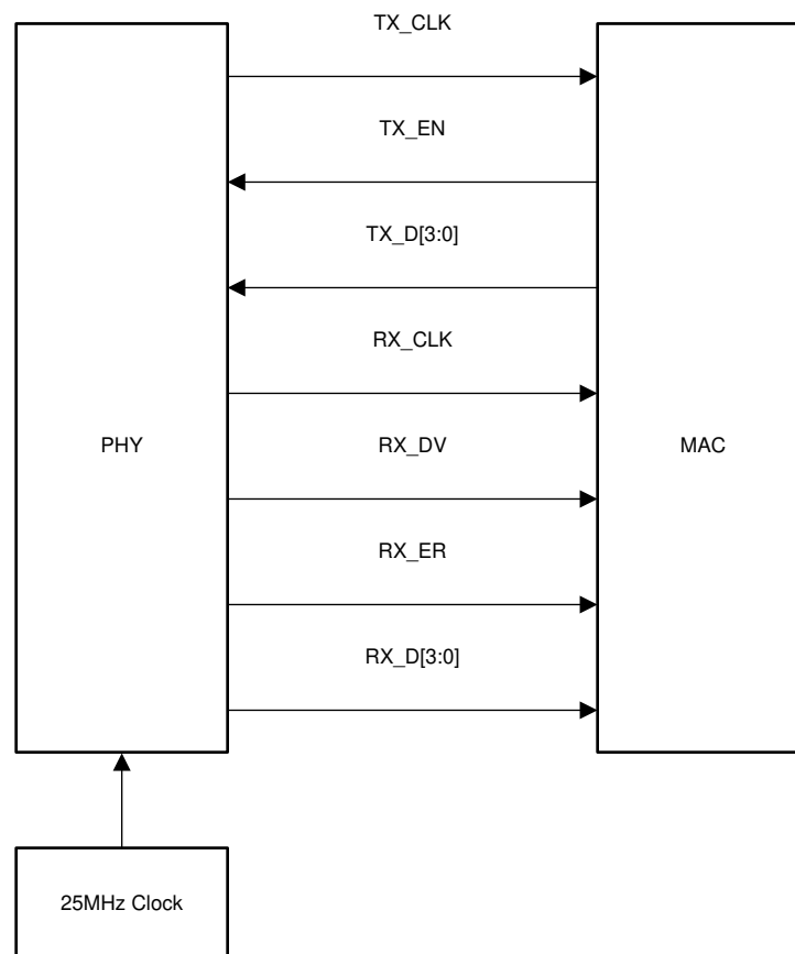
Figure 7-3. MII Signaling
