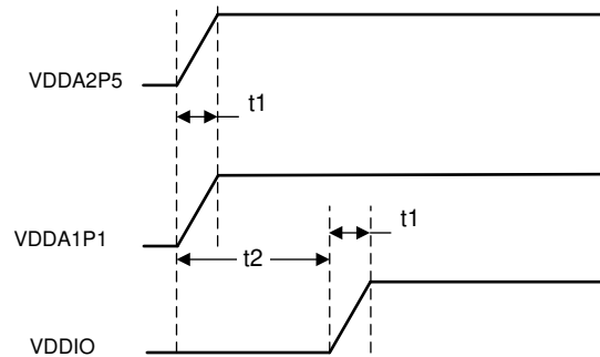
Figure 9-2. Two-Supply Sequence Diagram
