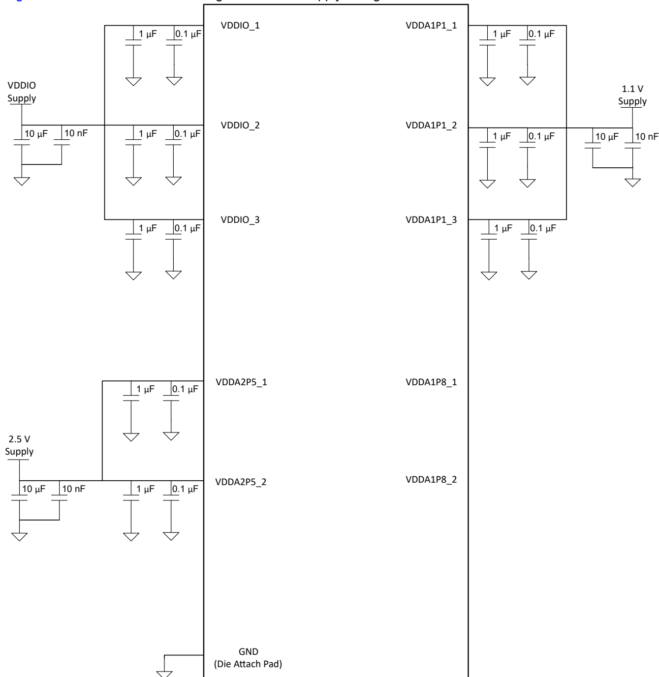
Figure 9-1. Two-Supply Configuration
