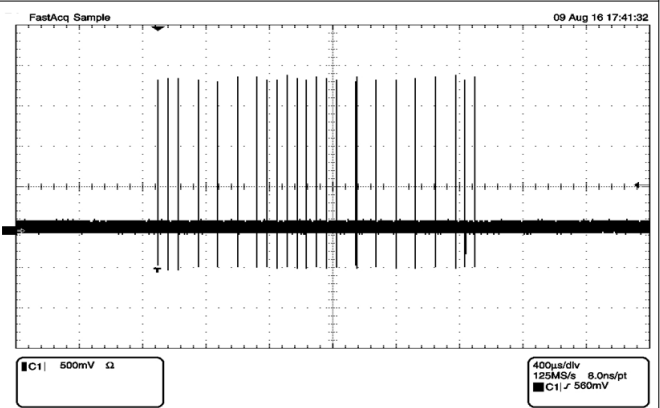
Figure 6-11. Auto-Negotiation FLP
