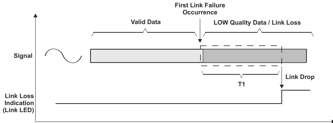
Figure 7-7. Fast Link Drop Mechanism
