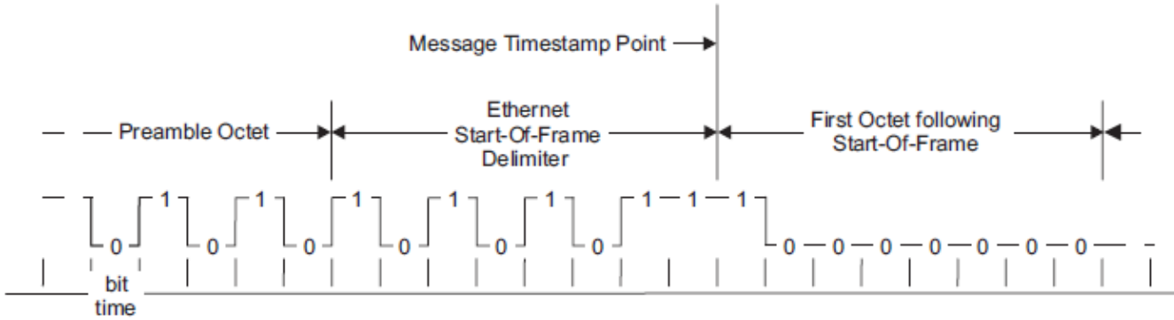
Figure 7-5. IEEE 1588 Message Timestamp Point
