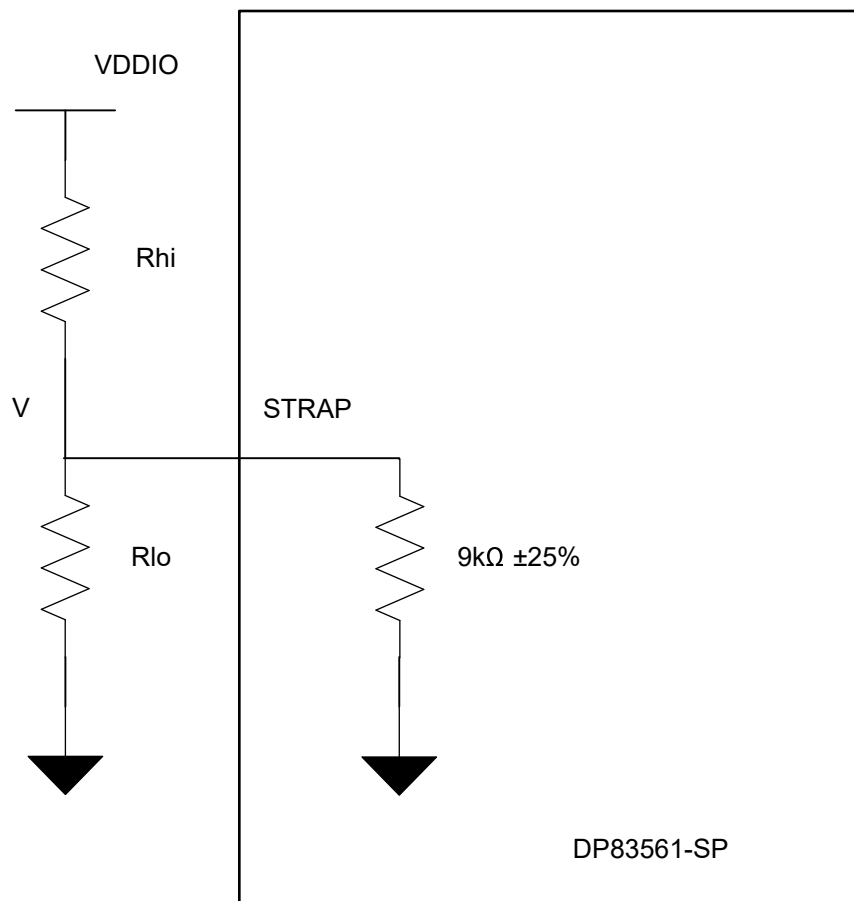
Figure 7-12. Strap Circuit
