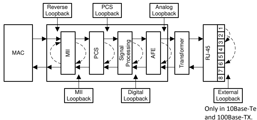
Figure 7-9. Loopbacks
