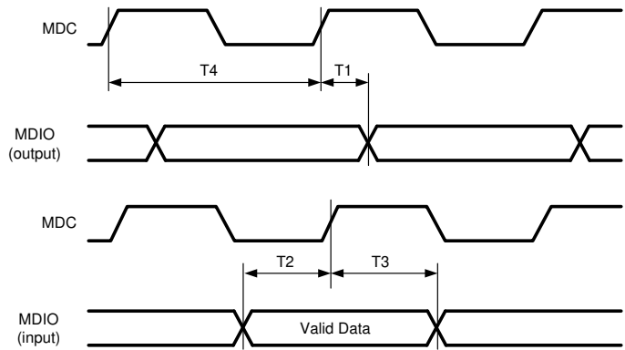
Figure 6-7. Serial Management Interface Timing
