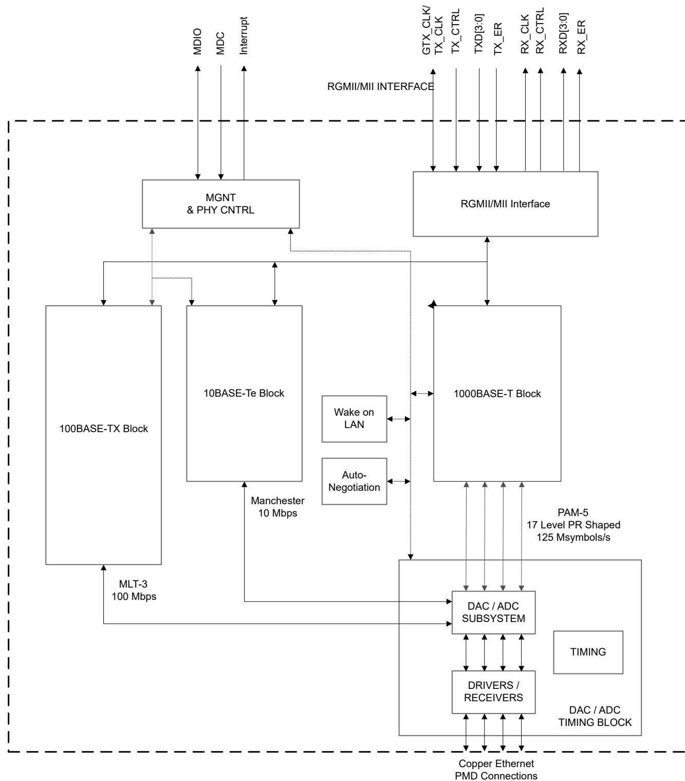
Figure 7-1. DP83561-SP Functional Block Diagram
