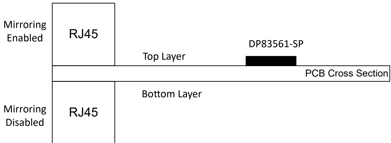
Figure 7-8. Normal and Mirror Mode RJ45 Mounting Orientation
