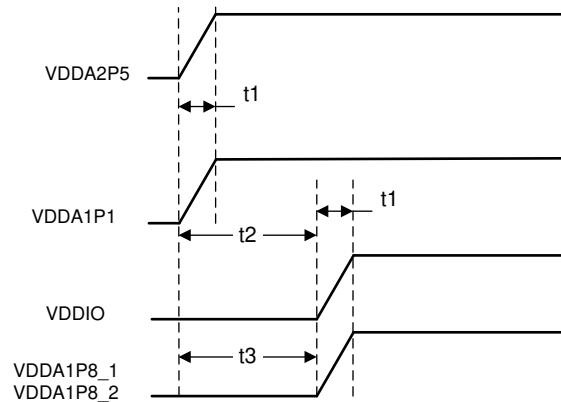
Figure 9-4. Three-Supply Sequence Diagram
