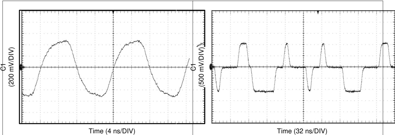
Figure 6-8. 1000Base-T Test Mode 2 Signal
