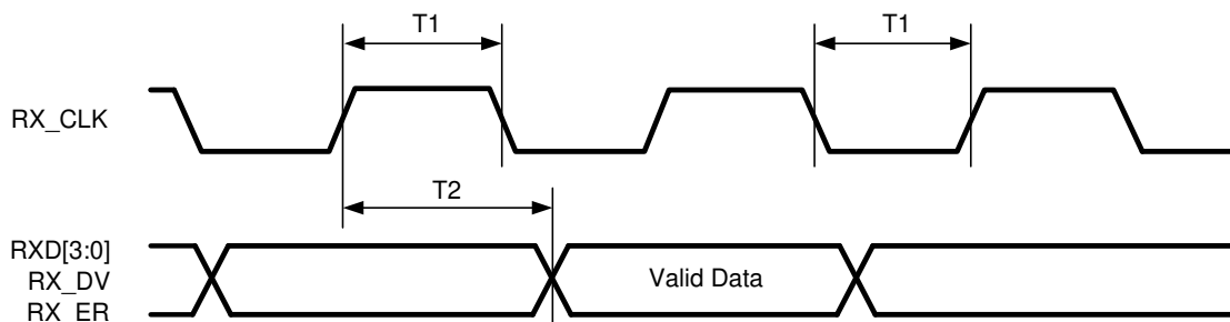
Figure 6-4. 100-Mbps MII Receive Timing
