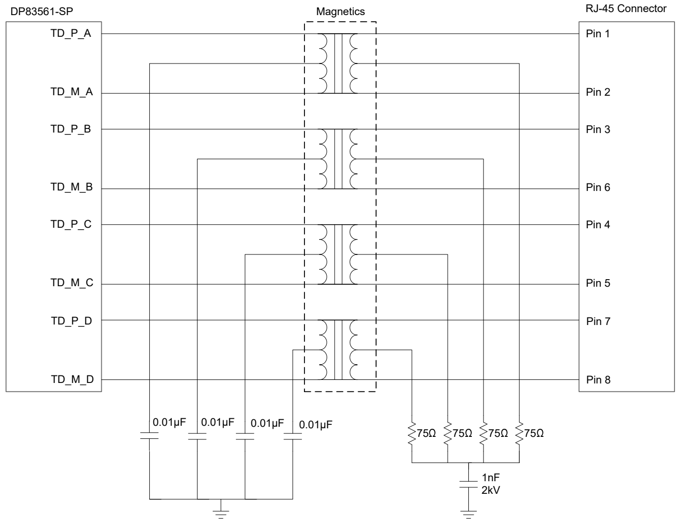
Figure 8-3. Magnetics Connection
