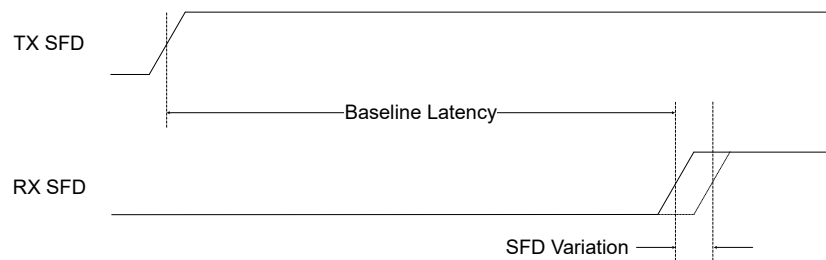
Figure 7-6. Baseline Latency and SFD Variation in Latency Measurement
