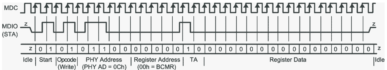
Figure 7-11. Typical MDC/MDIO Write Operation
