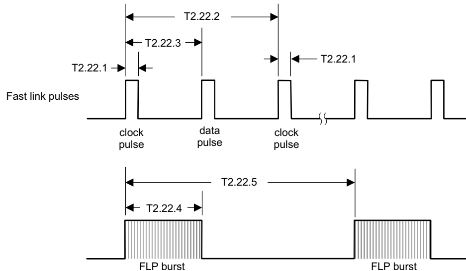
图 4-23. Auto-Negotiation Fast Link Pulse (FLP) Timing
