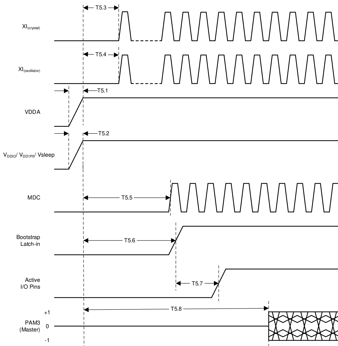
Figure 7-1. Power Up Timing
