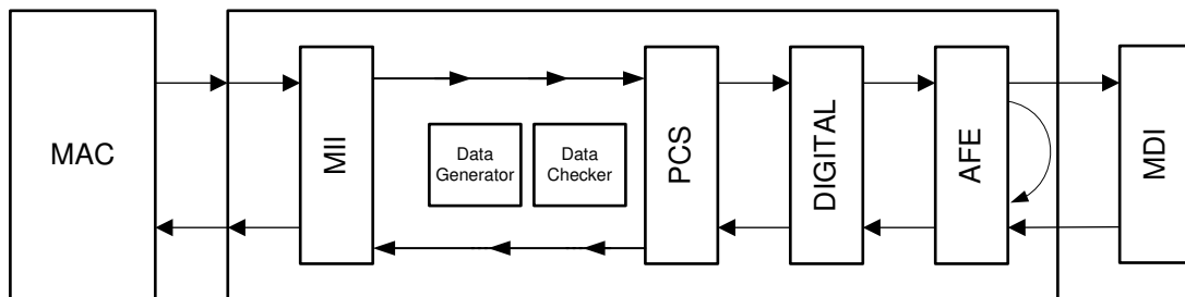
Figure 8-2. All Loopbacks
