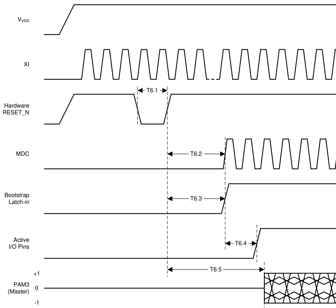
Figure 7-2. Reset Timing
