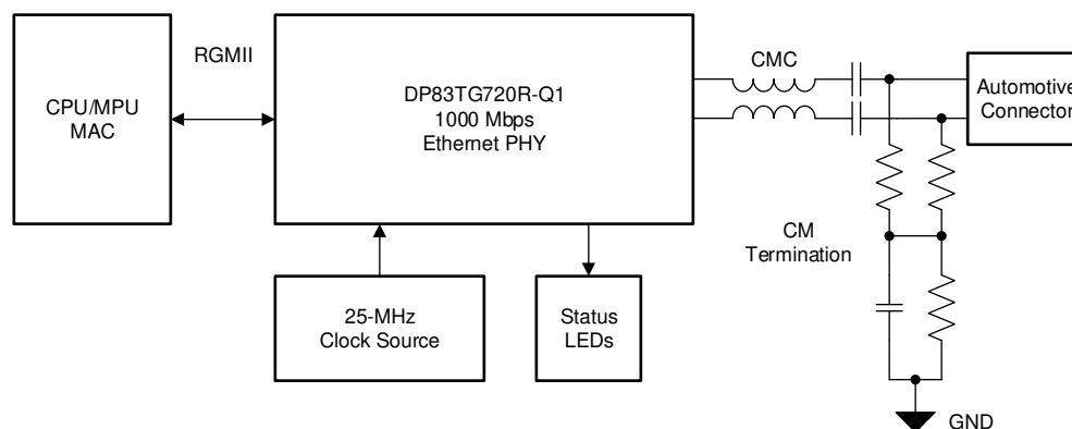
Figure 3-1. Simplified Schematic
