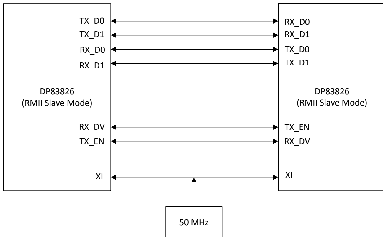
图 18. RMII Repeater Mode: Slave-Slave
