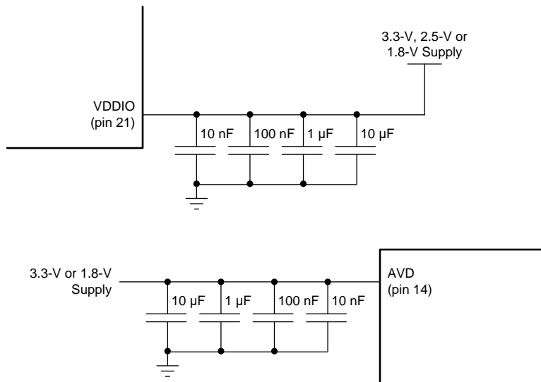
图 36. Power Connections
