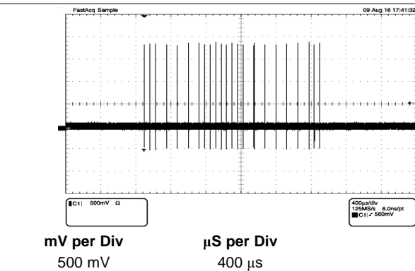
图 20. Auto-Negotiation Fast Link Pulses Waveform
