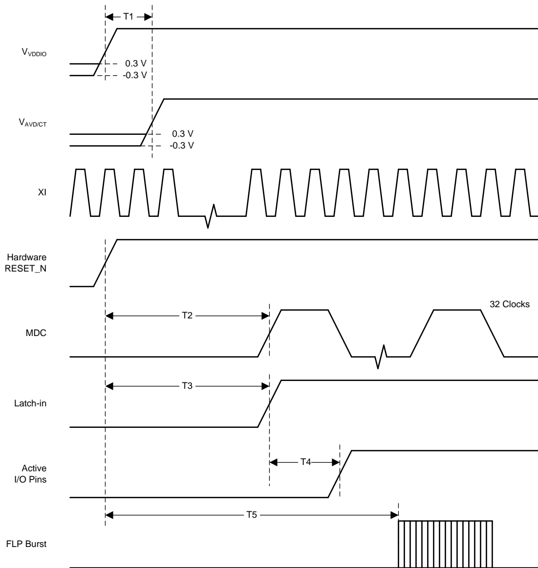
图 1. Power-Up Timing
