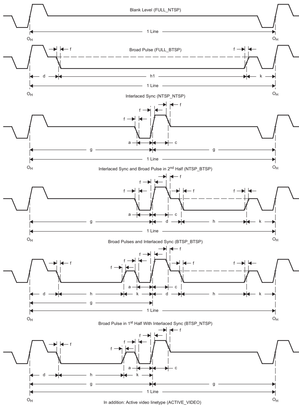
Figure 4-17. THS8200 VBI Line Types in HDTV Mode
