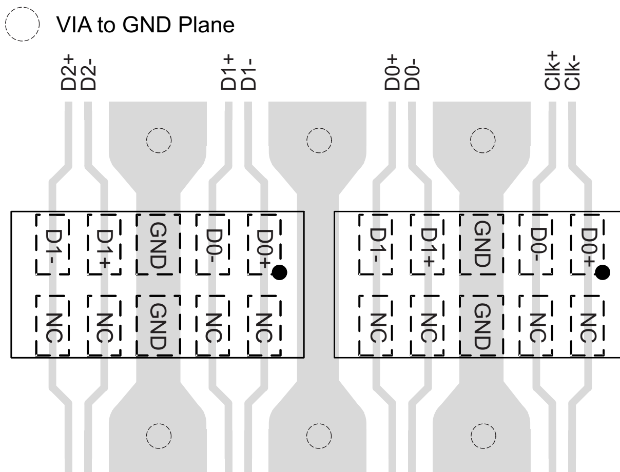
Figure 24. TPD4E05U06 Layout
