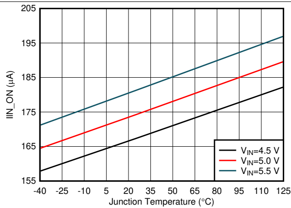
Figure 7. Enabled IN Supply Current vs Temperature
