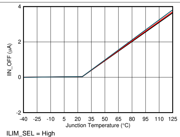
Figure 6. Disabled IN Supply Current vs Temperature
