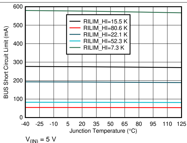
Figure 5. VBUS Short-Circuit Current Limit vs Temperature
