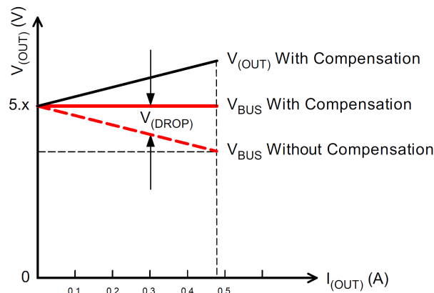
Figure 31. Voltage Drop
