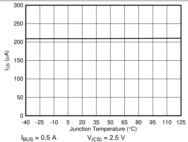
Figure 10. I_{CS} vs Temperature
