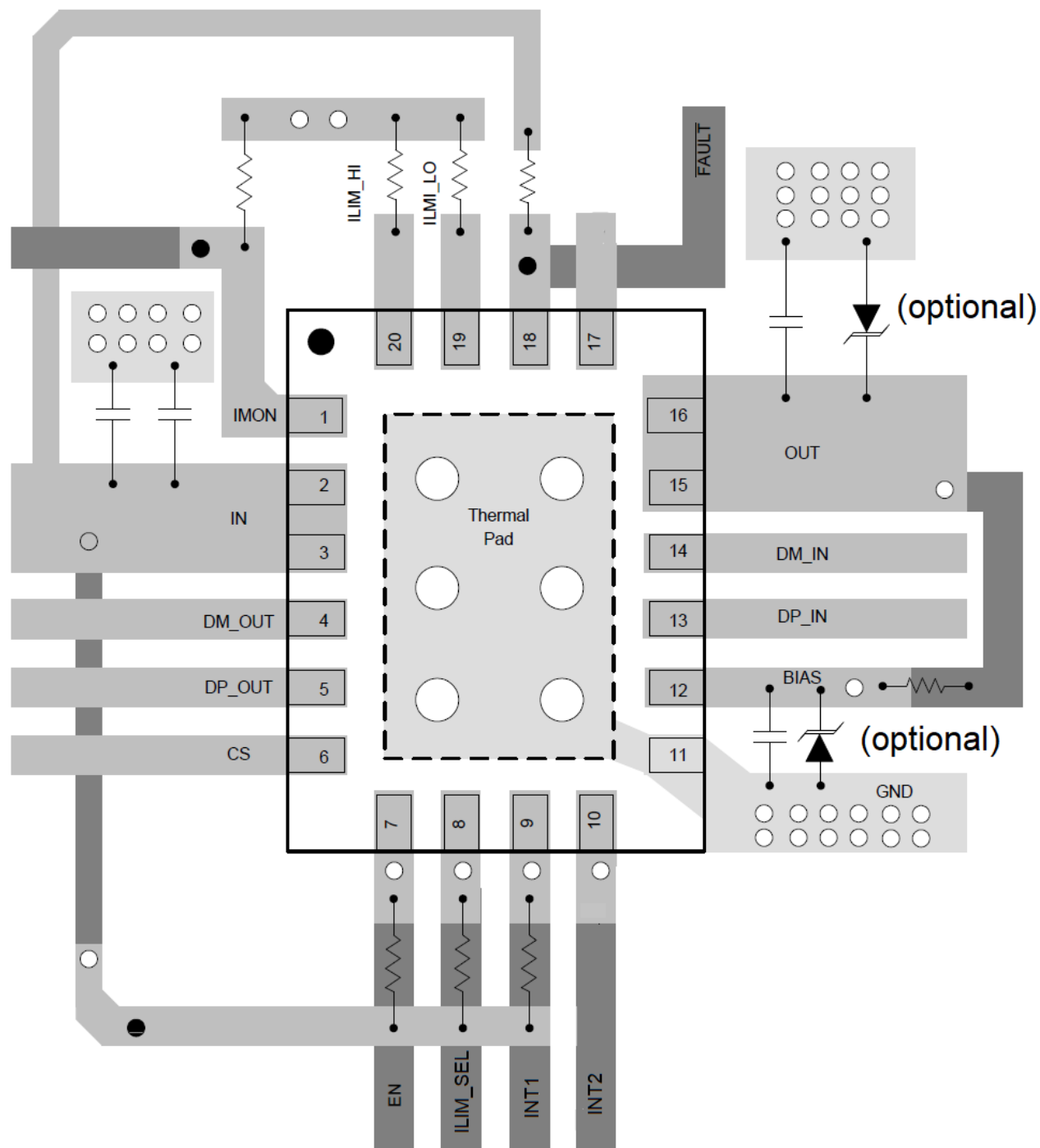
Figure 45. TPD3S713-Q1 Layout Diagram
