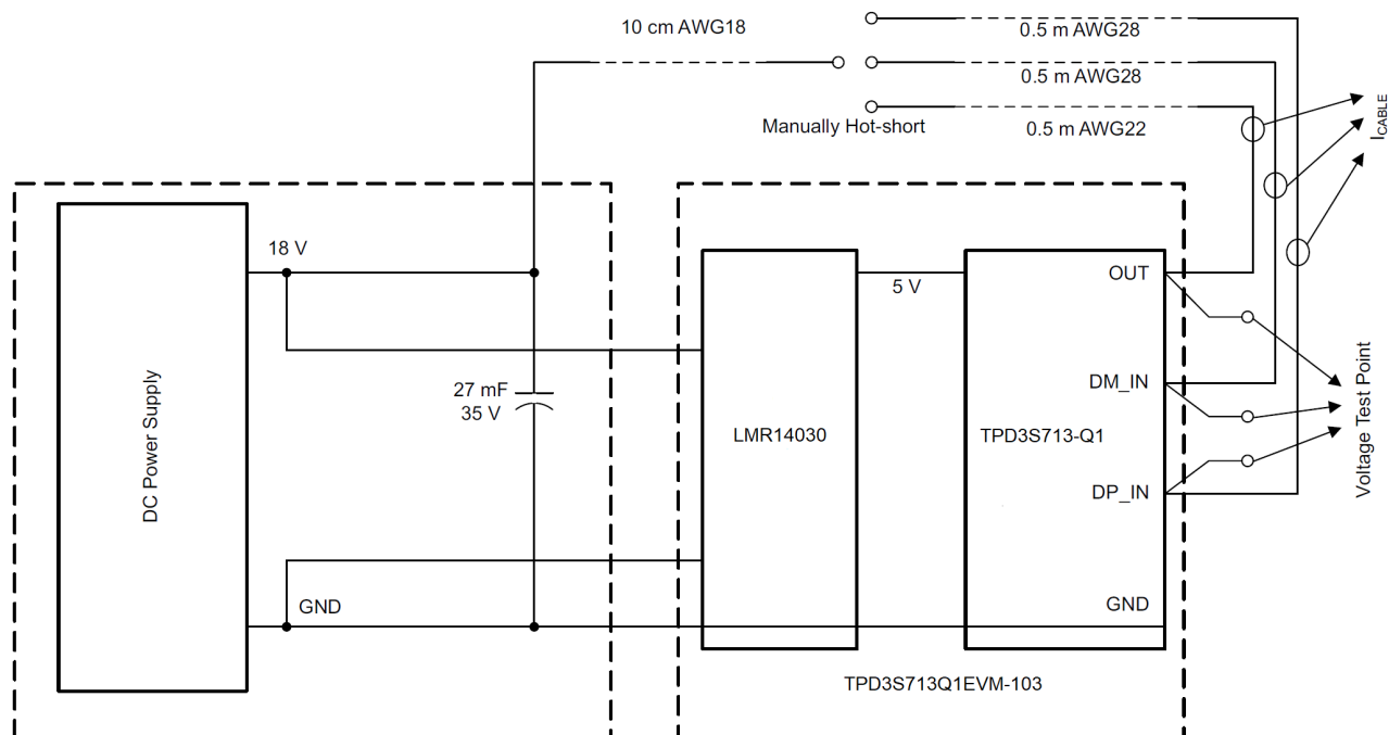
Figure 30. Short-to-Battery System Test Setup
