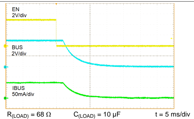
Figure 17. Turnoff Response
