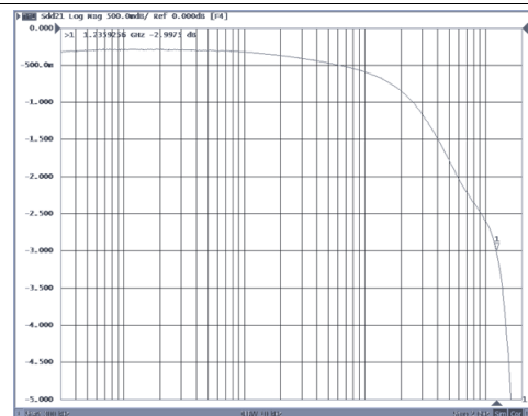
Figure 27. Data Transmission Characteristics vs Frequency
