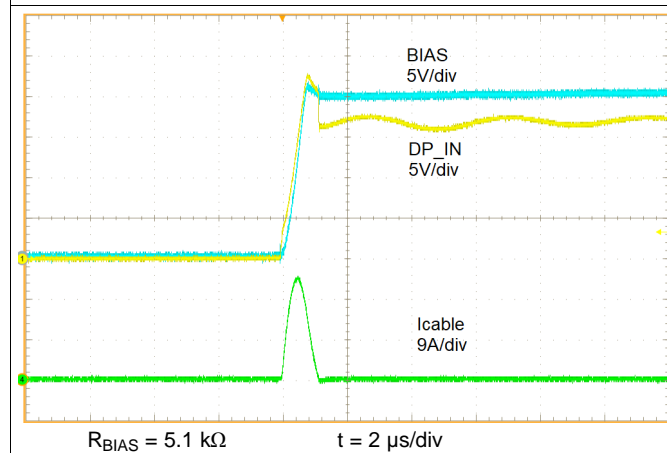
Figure 42. Disabled, DP_IN Shorted to Battery
