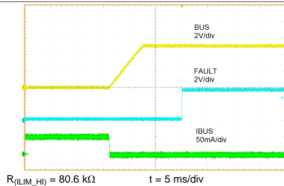
Figure 19. Short Circuit to No Load
