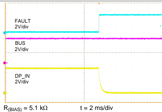
Figure 26. DP_IN Short-to- V_{BUS} and Recovery
