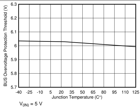
Figure 9. BUS Overvoltage Protection Threshold vs Temperature
