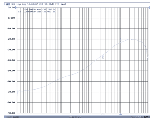
Figure 29. On-State Cross-Channel Isolation vs Frequency
