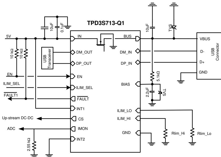
Figure 35. Typical Application Schematic
