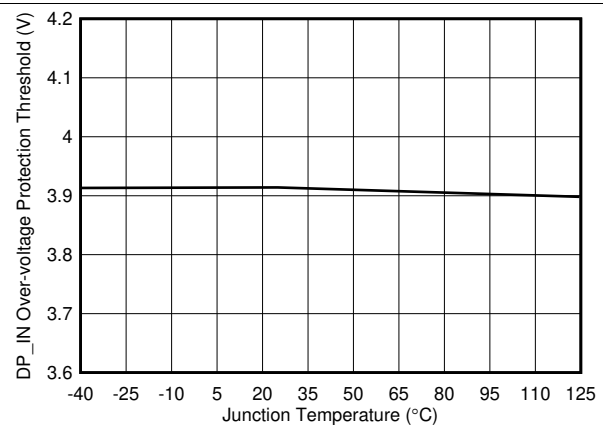
Figure 8. DP_IN Overvoltage Protection Threshold vs Temperature
