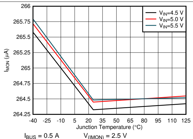
Figure 12. I_{IMON} vs Temperature
