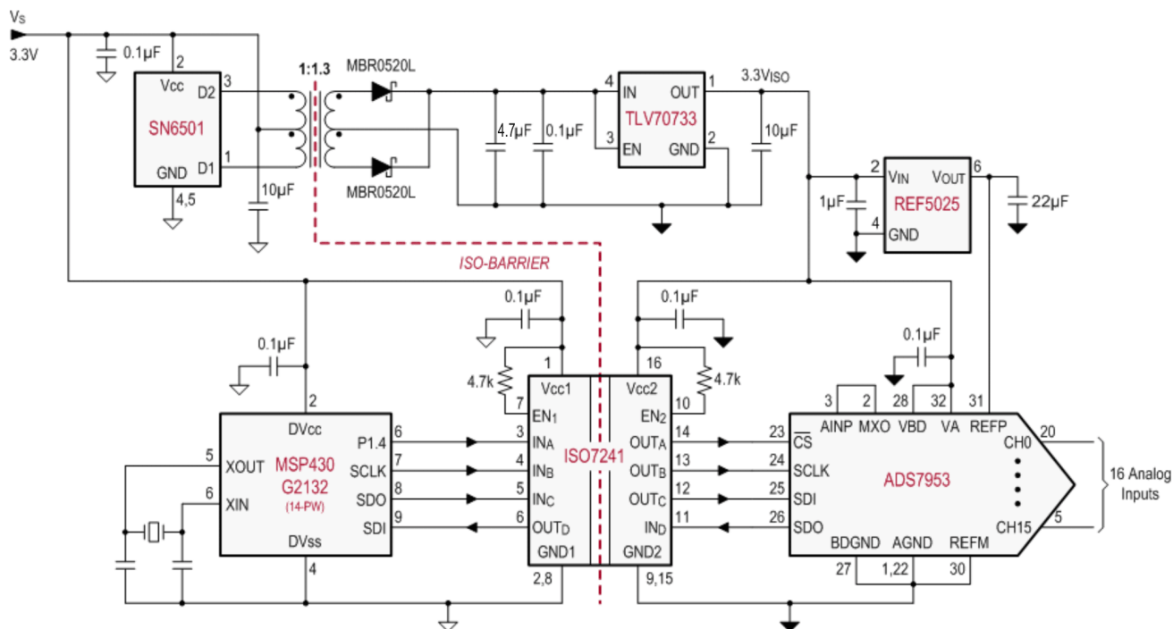
Figure 9-16. Isolated SPI Interface for an Analog Input Module With 16 Inputs
