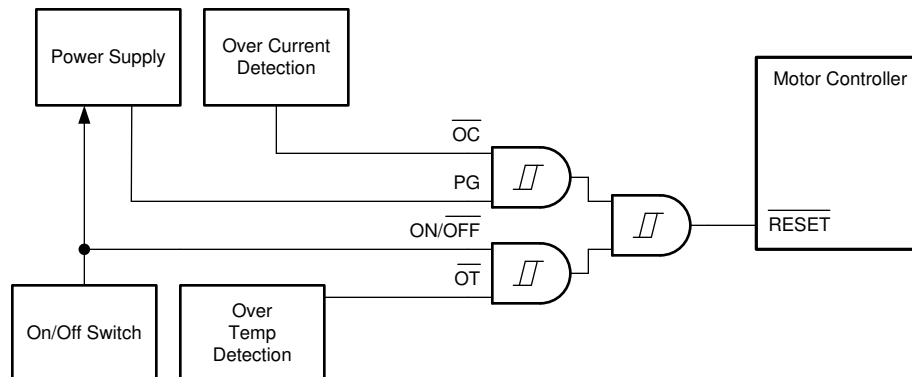
图 9. Typical application block diagram
