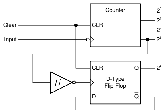
图 9. Typical application block diagram
