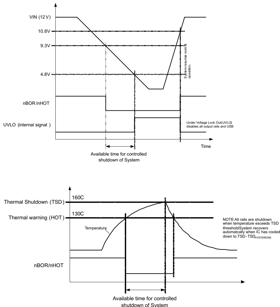
Figure 3. Brownout Monitoring
