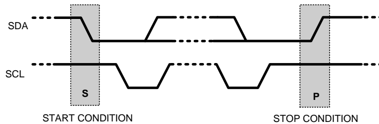
Figure 16. Start and Stop Conditions
