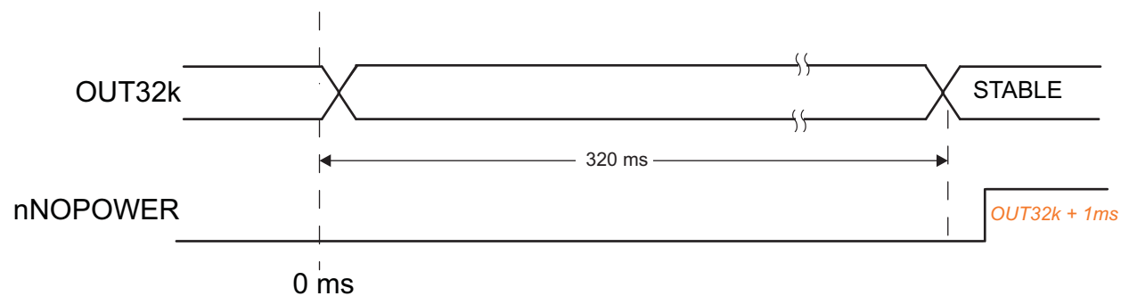
Figure 4-6. Sequence Timing
