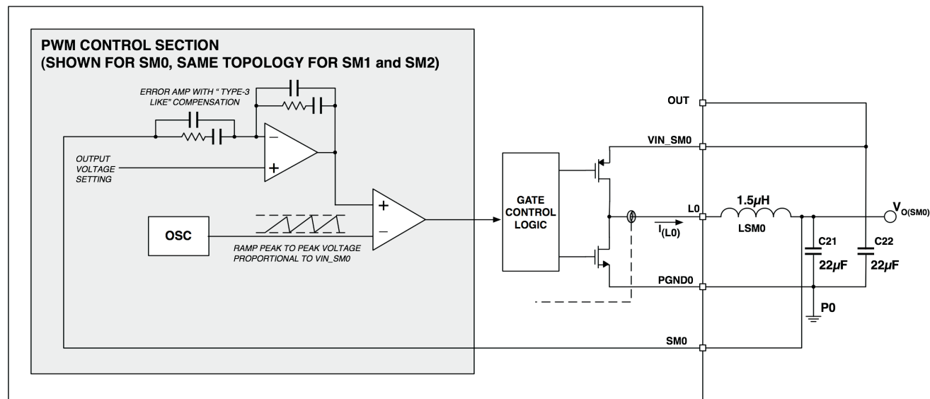
Figure 3-11. PWM Control
