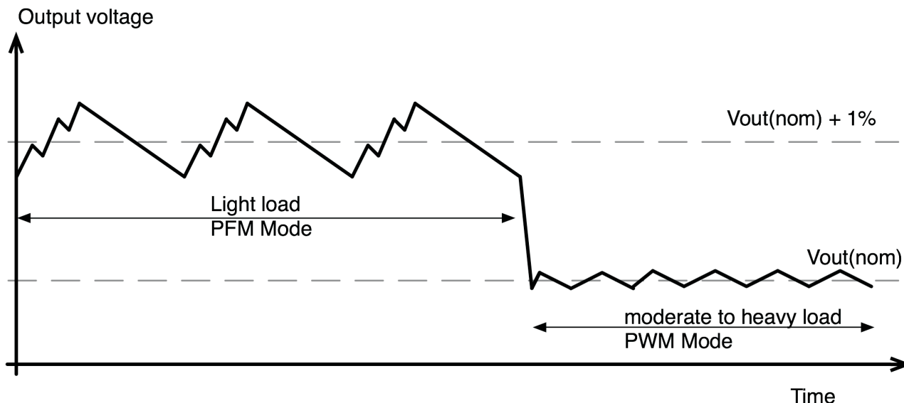
Figure 3-12. Voltage Positioning
