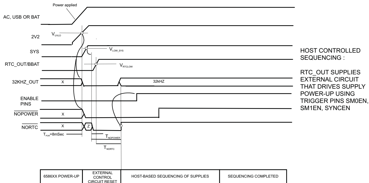
Figure 3-7. Host Controlled Startup
