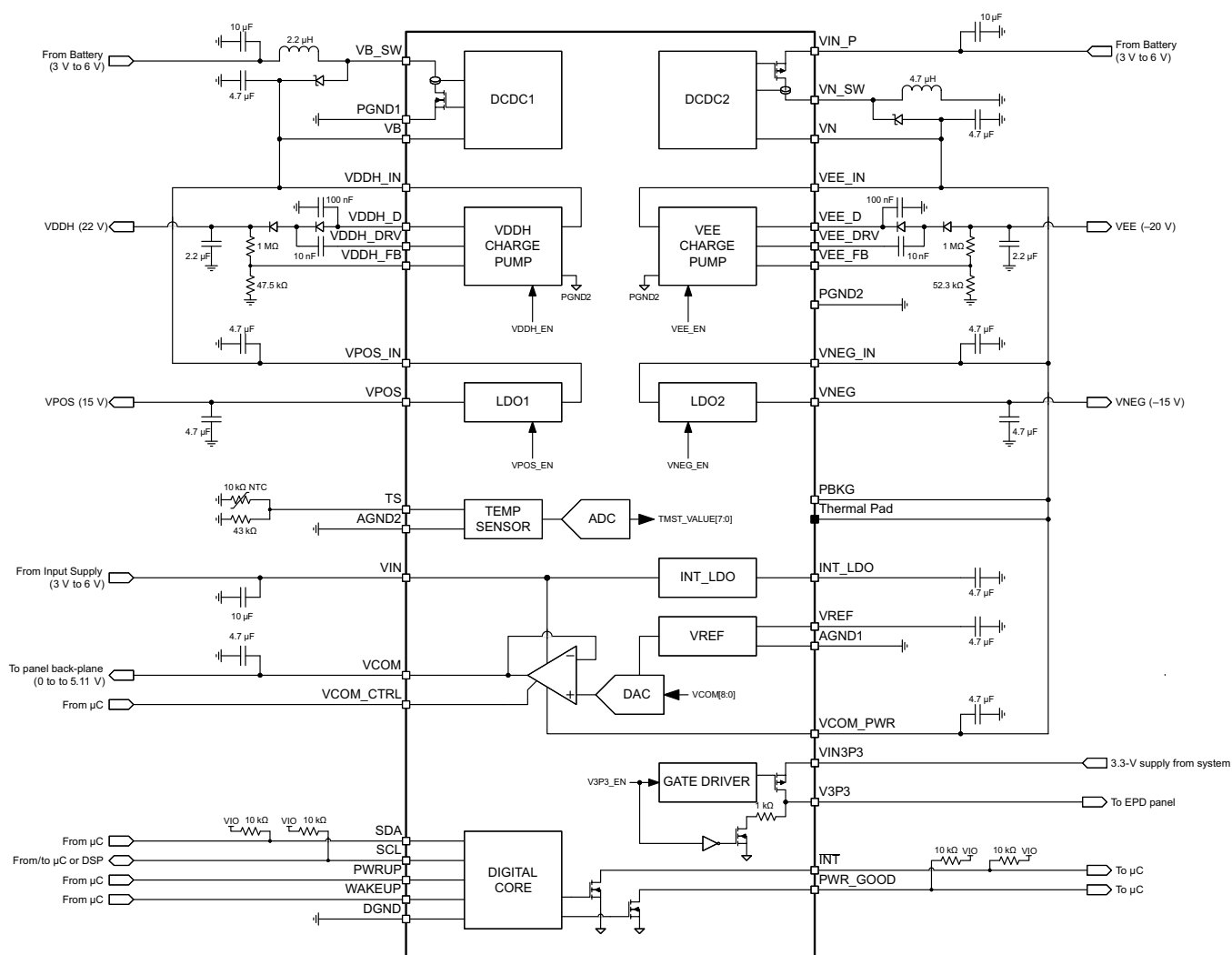
Figure 46. Typical Application Schematic
