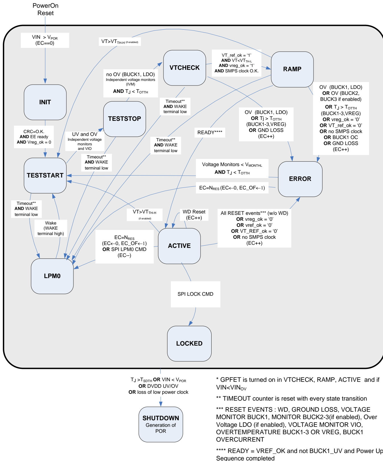
Figure 18. Operating Mode Transitions
