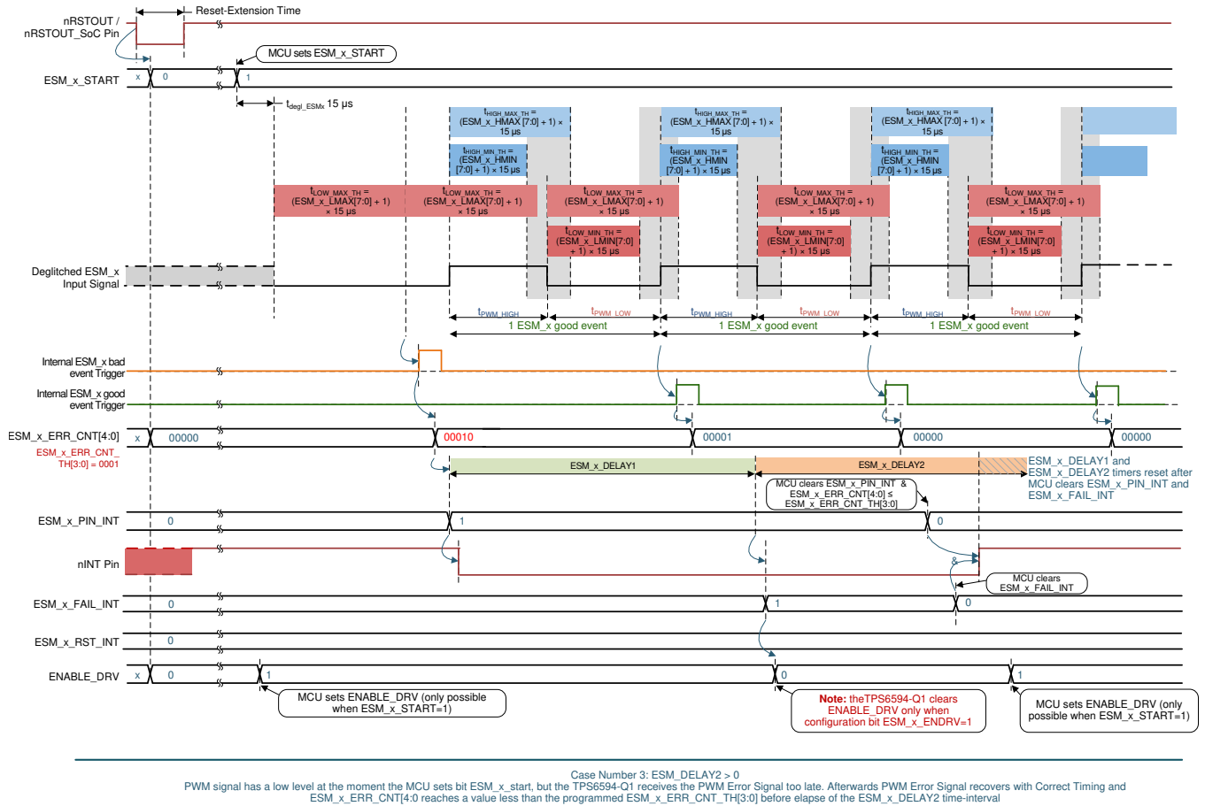
Figure 5-40. Example Waveform for ESM in PWM Mode - Case Number 3: ESM starts with low-level at deglitched input signal, but receives too late a correct PWM signal afterwards
