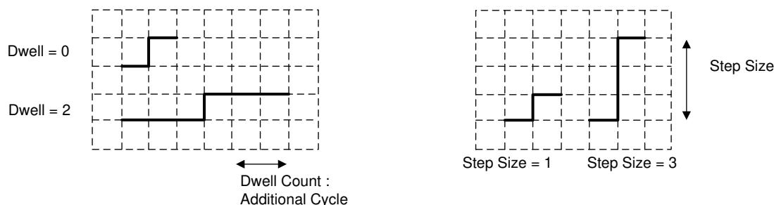
Figure 5-5. Internal Spread-Spectrum Configuration Options (Controlled through EEPROM-Mapped Bits)
