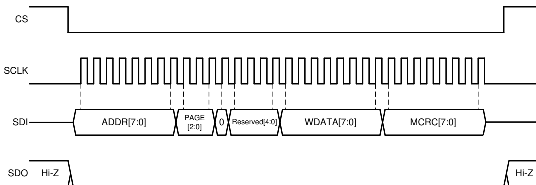
Figure 5-65. SPI Write Cycle with Master CRC
