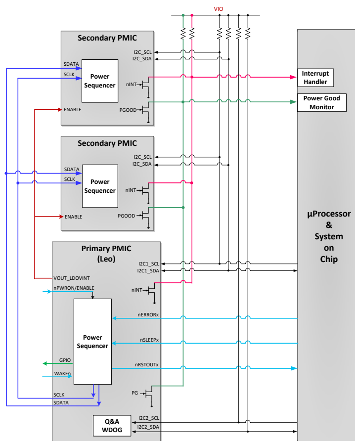
Figure 5-50. Multi-PMIC Pin Connections
