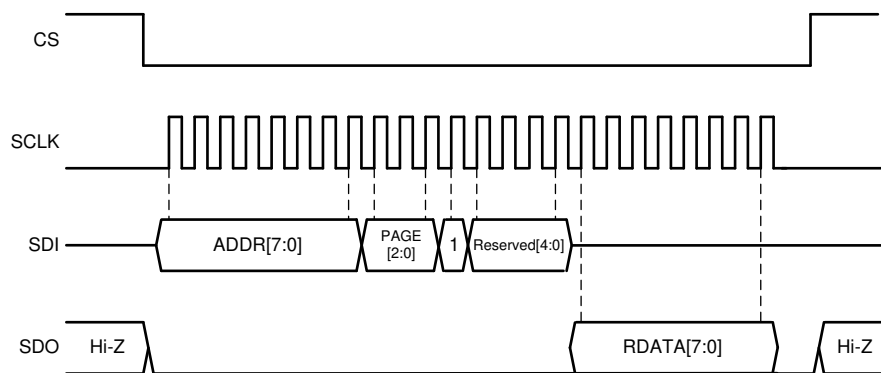
Figure 5-66. SPI Read Cycle
