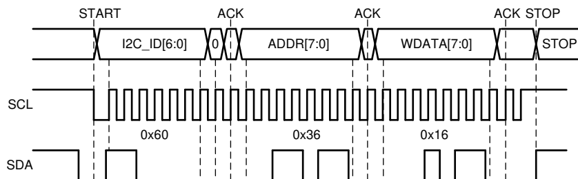
Figure 5-60. I²C Write Cycle without CRC
