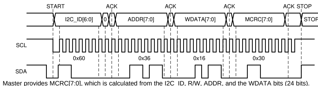
Figure 5-61. I²C Write Cycle with CRC
