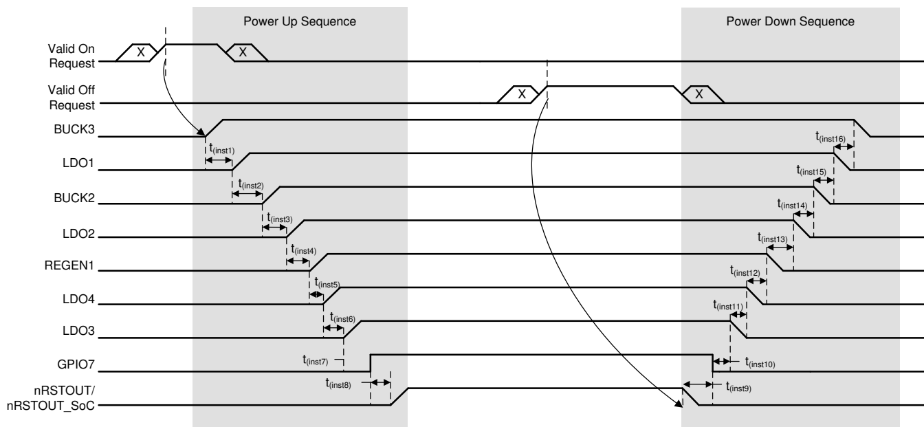
Figure 5-48. Power Sequence Example
