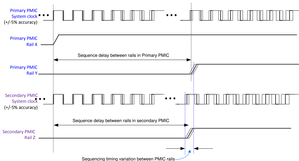
Figure 5-51. Multi-PMIC Rail Sequencing Timing Variation
