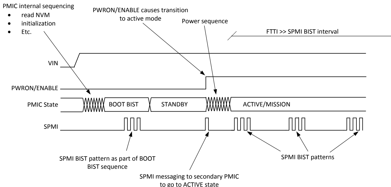
Figure 5-53. SPMI BIST Operation
