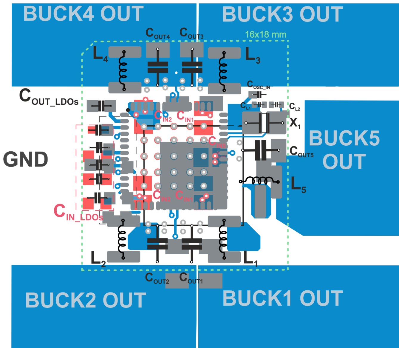
Figure 6-4. Example PMIC Layout
