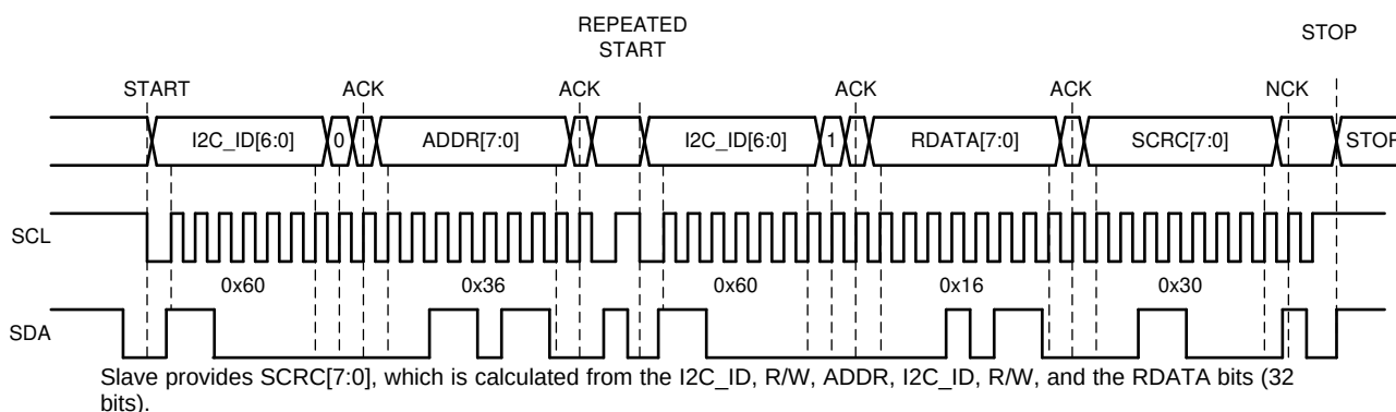
Figure 5-63. I²C READ Cycle with CRC
