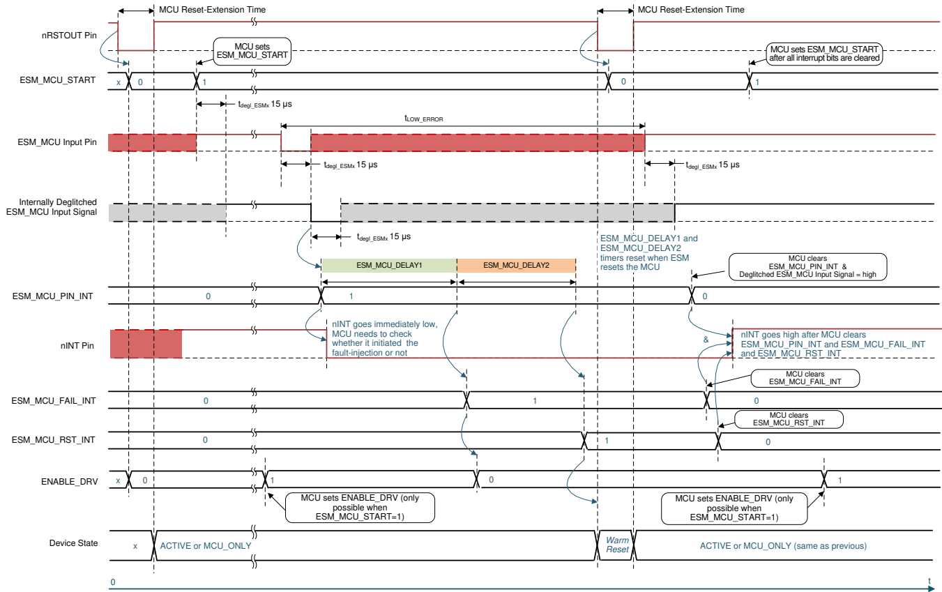
Figure 5-36. Example Waveform for ESM in Level Mode - Case Number 3b: Delay-2 not set to 0 and ESM_MCU_ENDRV=1, ESM_MCU input signal recovers too late and MCU-reset occurs
