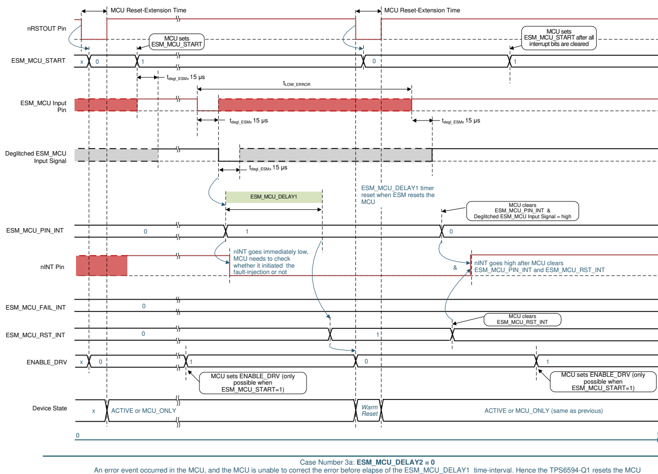
Figure 5-35. Example Waveform for ESM in Level Mode - Case Number 3a: Delay-2 set to 0 and ESM_MCU_ENDRV=1, ESM_MCU input signal recovers too late and MCU-reset occurs
