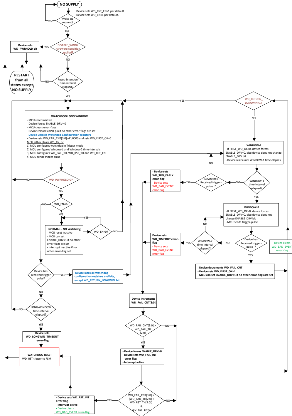
Figure 5-22. Flow Chart for WatchDog Monitor in Trigger Mode
