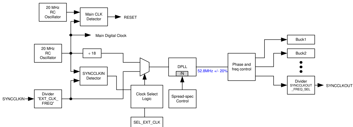
图 5-12. Sync Clock and DPLL Module
