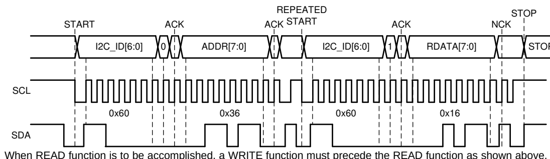
Figure 5-62. I²C Read Cycle without CRC
