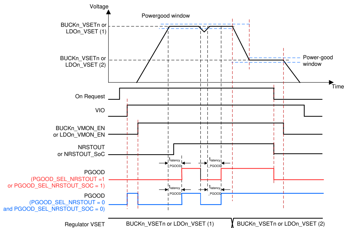
Figure 5-16. PGOOD Waveforms
