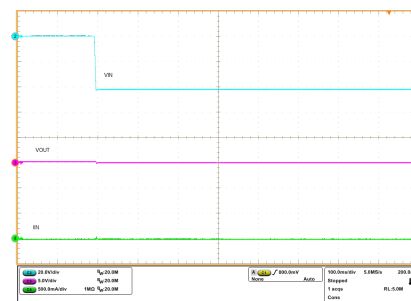
Reverse Polarity Protection with -42\text{ V} Input
