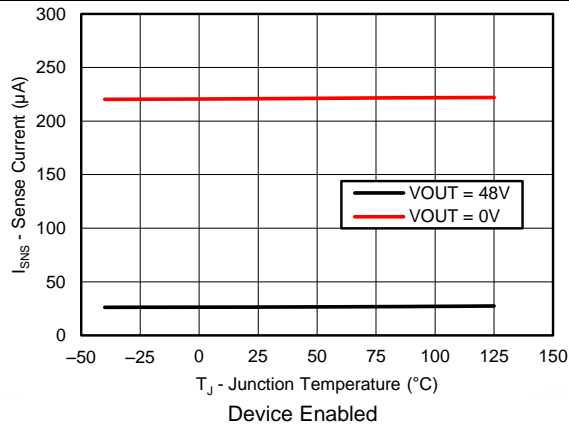
图 3. Sense Current vs VOUT and T_J
