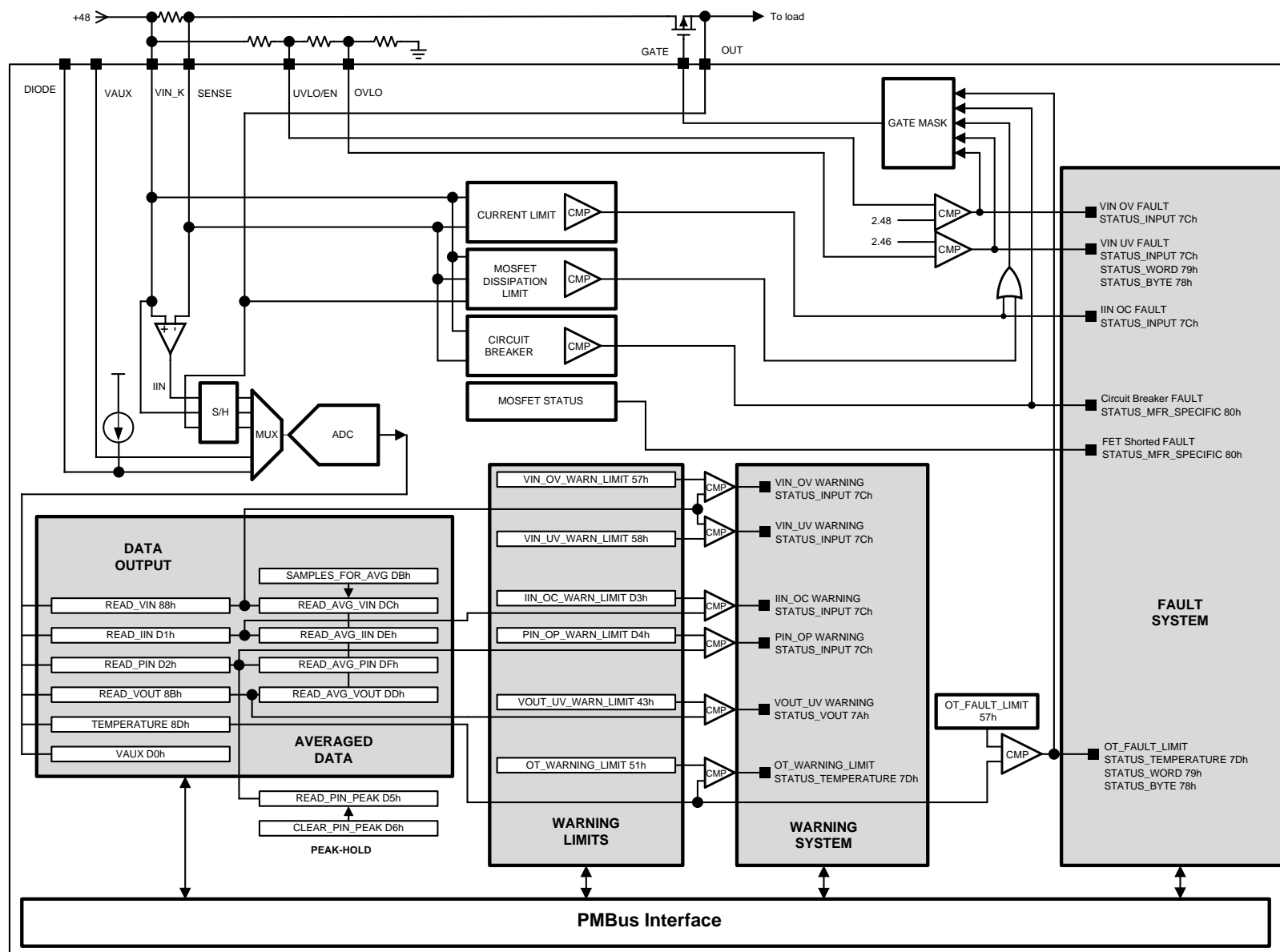
图 17. Command / Register and Alert Flow Diagram
