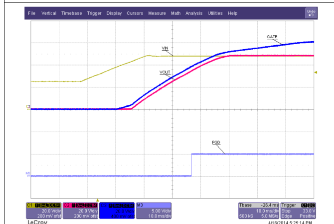
图 43. Start-Up
