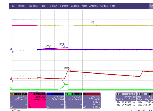
图 47. Gradual Overcurrent
