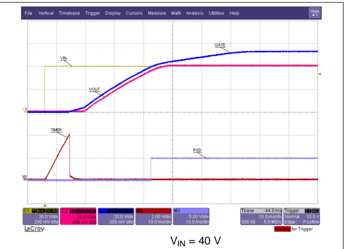
图 42. Start-Up
