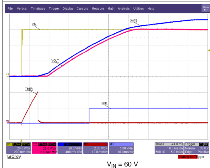
图 43. Start-Up
