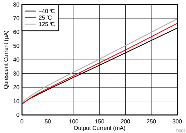
图 1. Ground Current vs Output Current
