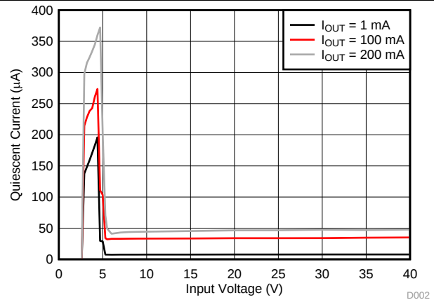
图 2. Ground Current vs Input Voltage
