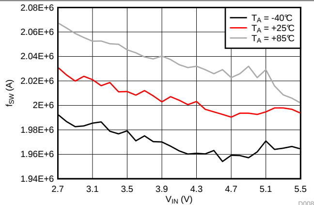
Figure 10. Switching Frequency
