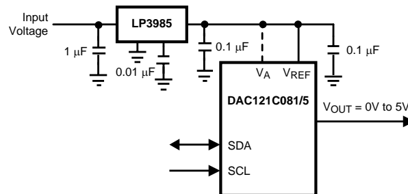
Figure 33. Using the LP3985 Regulator
