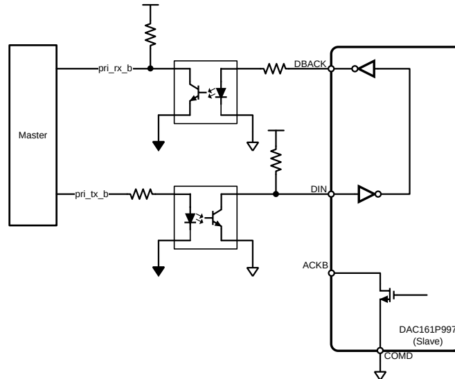
Figure 32. SWIF Link Realized With Octo-Couplers
