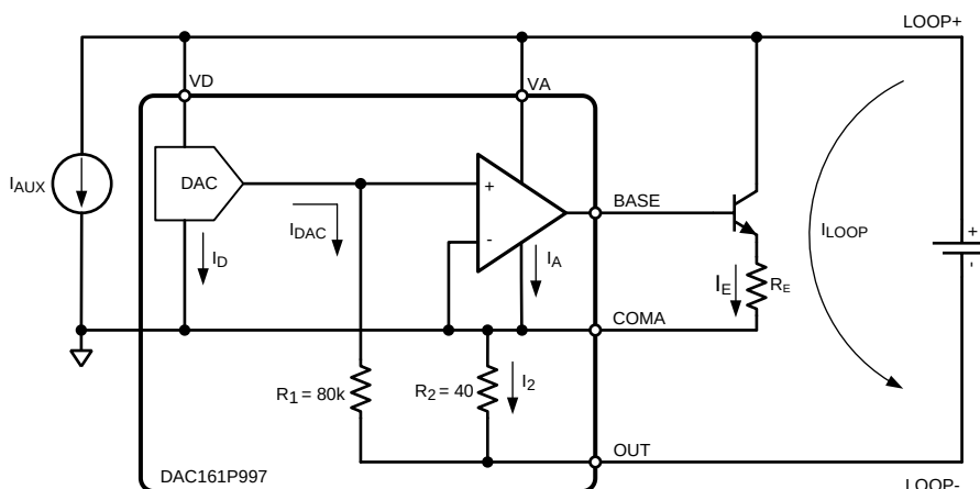
Figure 21. Loop-Powered Transmitter
