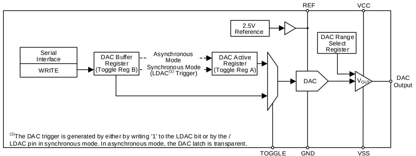
图 47. DACx1416 DAC Block Diagram
