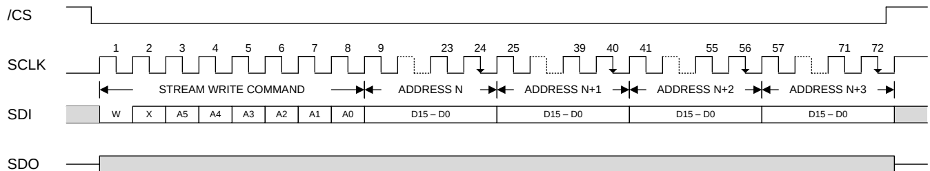
图 50. Serial Interface Streaming Cycle
