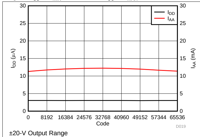
图 19. Supply Current ( I_{DD} , I_{AA} ) vs Digital Input Code
