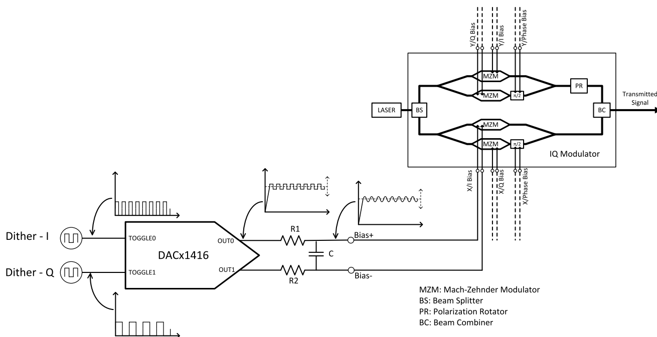
图 67. Biasing a Mach Zehnder Modulator
