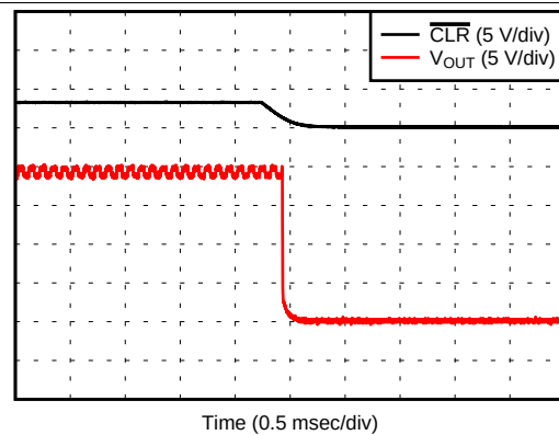
图 34. Power-Down Response
