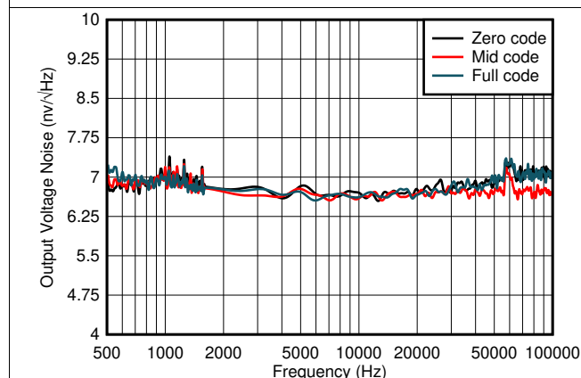
图 41. DAC Output Noise Spectral Density
