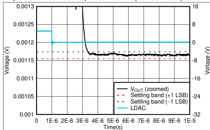
图 39. 100 Codes Settling Time, Falling Edge
