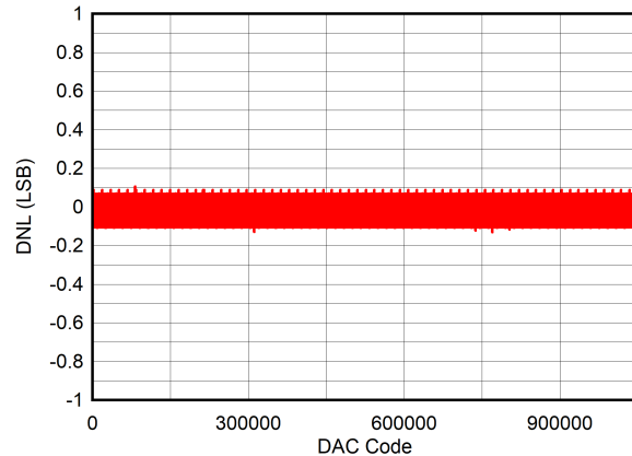
图 58. DNL at \pm 10 -V Output
