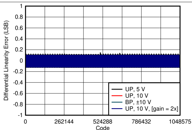
图 4. Differential Linearity Error vs Digital Input Code
