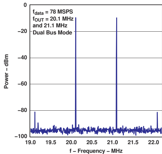
图 6-11. Two-Tone Spectrum
