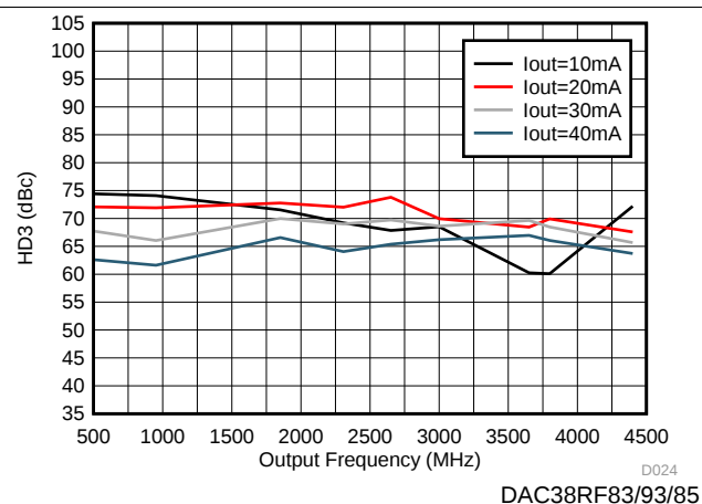
Figure 15. HD3 vs Output Frequency Over Output Current I_{outFS}
