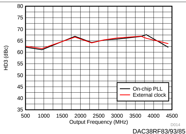
Figure 17. HD3 vs Output Frequency Over Clocking Option
