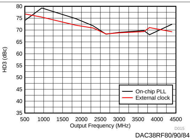
Figure 18. HD3 vs Output Frequency Over Clocking Option
