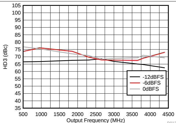
Figure 14. HD3 vs Output Frequency Over Input Scale
