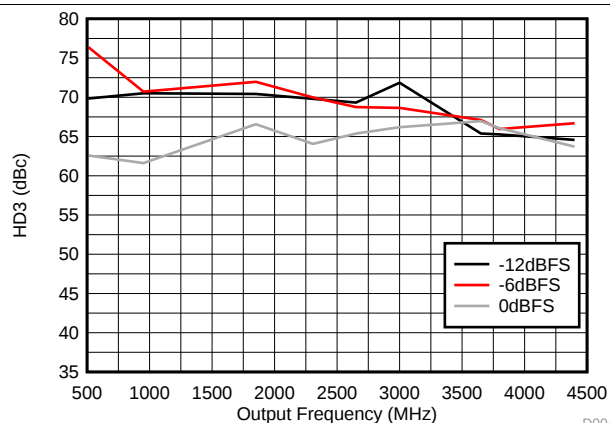
Figure 13. HD3 vs Output Frequency Over Input Scale
