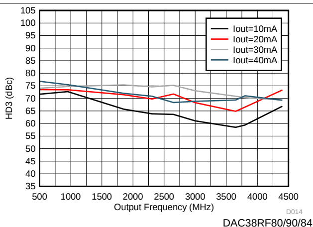
Figure 16. HD3 vs Output Frequency Over Output Current I_{outFS}
