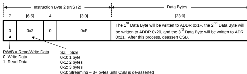
Figure 67. Register-Write Example 1
