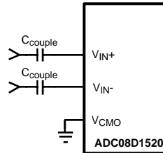
Figure 37. V_{CMO} Drive for A.C. Coupled Differential Input
