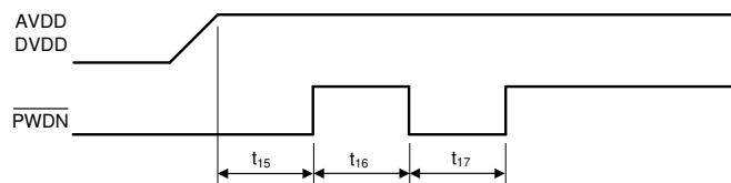
图 8-15. Power-Up Timing Sequence
