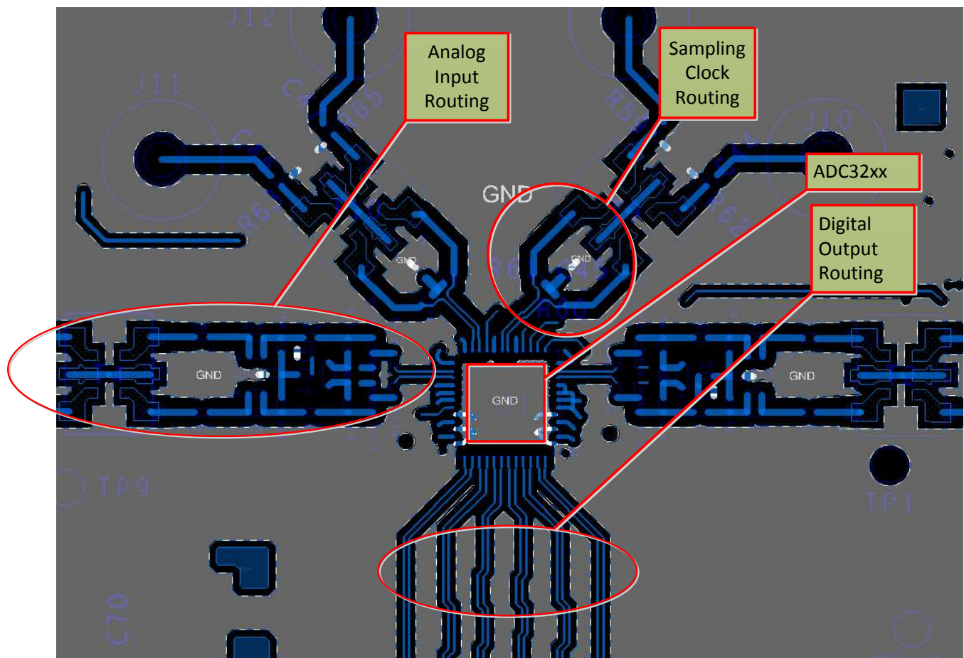
Figure 184. Typical Layout of the ADC324x Board
