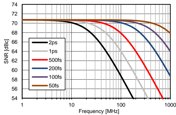
图 48. SNR Limit Due to Jitter of Sampling Clock With a Full-Scale Input Signal
