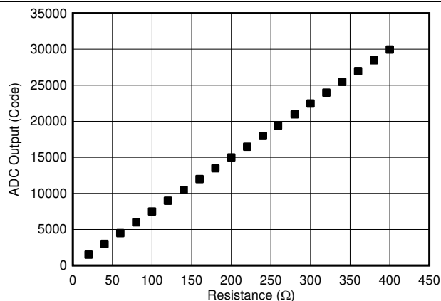
图 97. ADC Output Code vs Equivalent RTD Resistance
