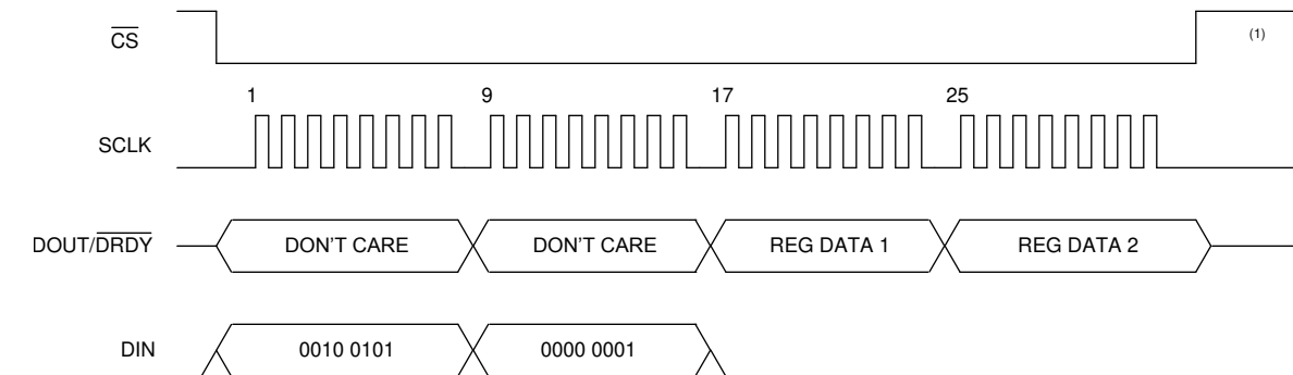
图 74. Read Register Sequence
