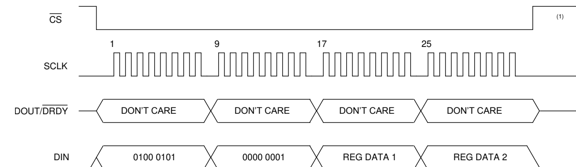
图 75. Write Register Sequence
