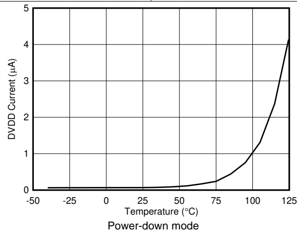
图 41. Digital Supply Current vs Temperature
