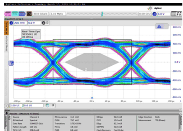
图 8-24. Eye at 5-Gbps Bit Rate with Increased Output Swing
