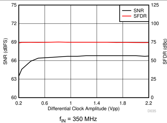
图 7-41. Performance vs Sampling Clock Amplitude
