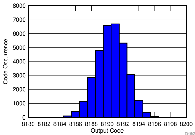
图 9-8. Idle Channel Histogram (No Signal at Analog Inputs, DC Offset Correction is Frozen)
