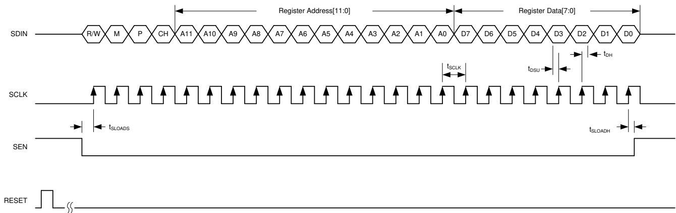
图 8-12. SPI Timing Diagram
