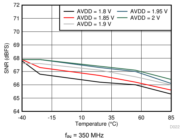
图 7-25. Signal-to-Noise Ratio vs AVDD Supply and Temperature
