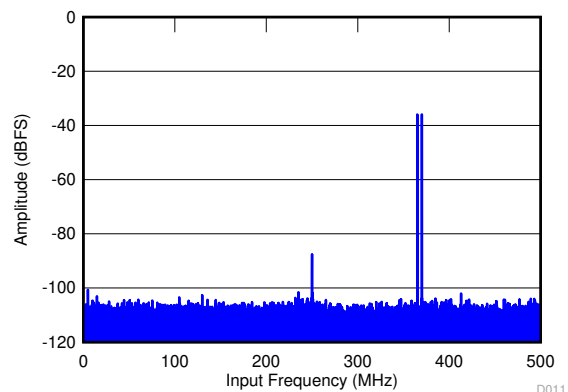
图 7-12. FFT for Two-Tone Input Signal ( - 36 dBFS)
