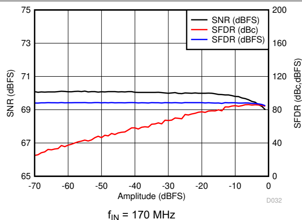
图 7-38. Performance vs Input Amplitude
