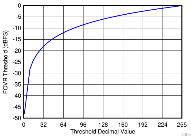
图 8-11. Programming Fast OVR Thresholds
