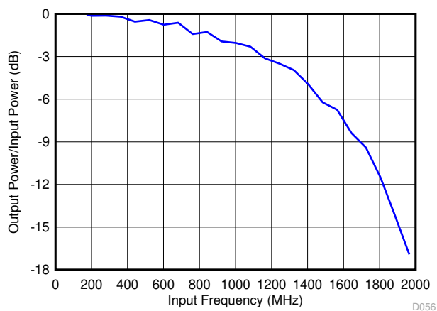
图 8-2. Transfer Function vs Frequency
