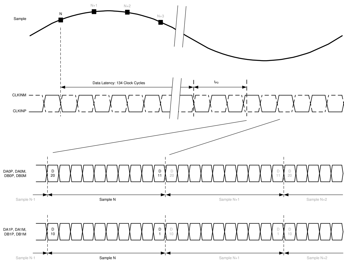
图 7-2. Sample Timing Requirements
