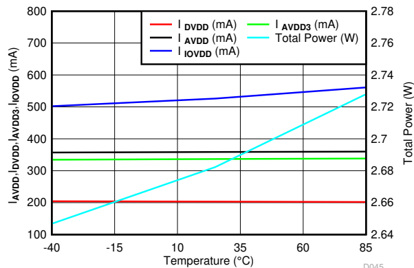
图 7-49. Power vs Temperature
