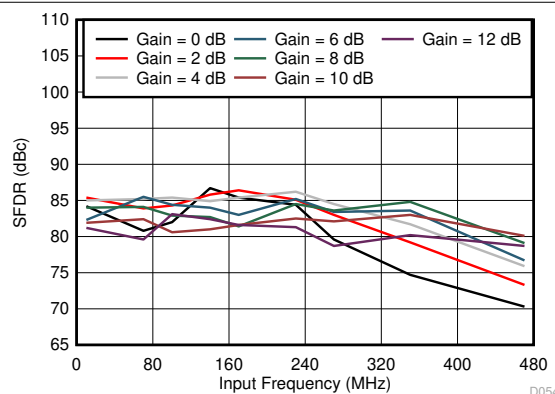
图 7-36. Spurious-Free Dynamic Range vs Gain and Input Frequency
