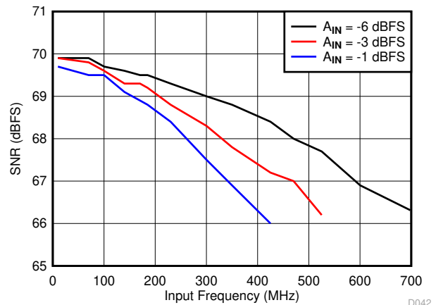
图 7-22. Signal-to-Noise Ratio vs Input Frequency
