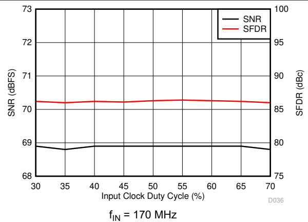
图 7-42. Performance vs Input Clock Duty Cycle
