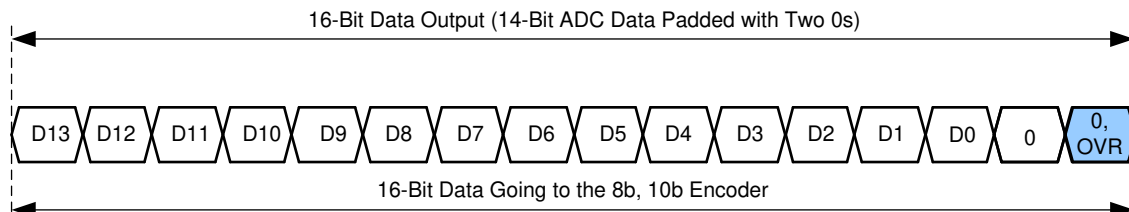
图 8-10. Overrange Indication in a Data Stream
