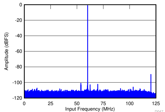
图 7-50. FFT for 60-MHz Input Signal in Decimate-by-4 Mode
