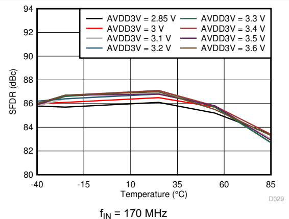
图 7-32. Spurious-Free Dynamic Range vs AVDD3V Supply and Temperature
