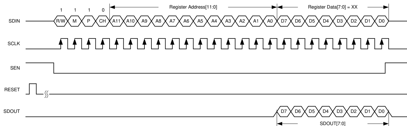
图 8-17. JESD Serial Register Read Timing Diagram
