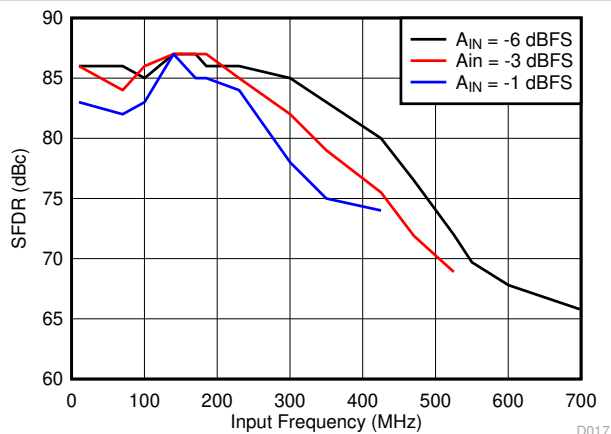
图 7-20. Spurious-Free Dynamic Range vs Input Frequency
