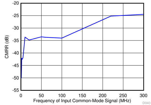
图 7-46. Common-Mode Rejection Ratio vs Test Signal Frequency
