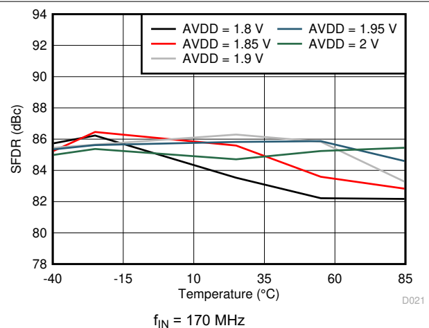
图 7-24. Spurious-Free Dynamic Range vs AVDD Supply and Temperature
