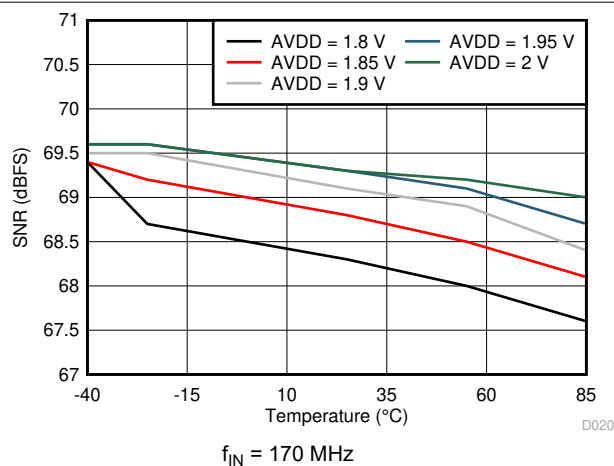
图 7-23. Signal-to-Noise Ratio vs AVDD Supply and Temperature
