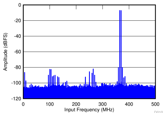
图 7-11. FFT for Two-Tone Input Signal ( - 7 dBFS)
