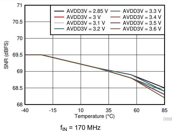
图 7-31. Signal-to-Noise Ratio vs AVDD3V Supply and Temperature
