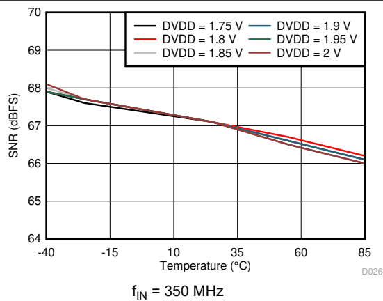
图 7-29. Signal-to-Noise Ratio vs DVDD Supply and Temperature
