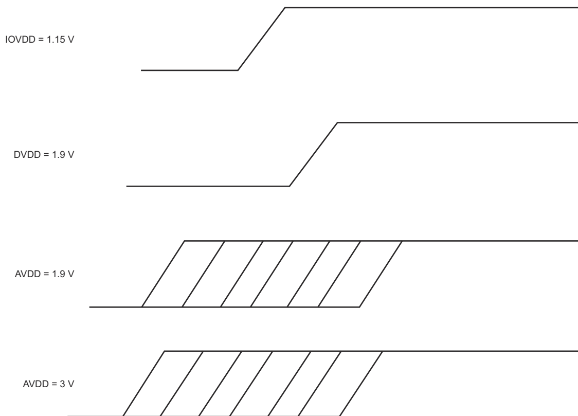
图 10-1. Power Sequencing for the ADS54Jxx Family of Devices
