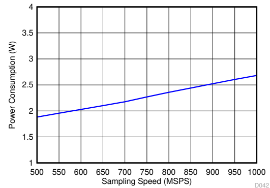
图 7-48. Power Consumption vs Sampling Speed
