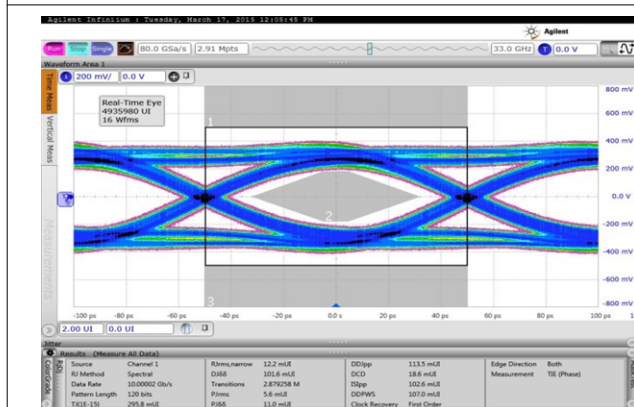
图 8-25. Eye at 10-Gbps Bit Rate with Default Output Swing
