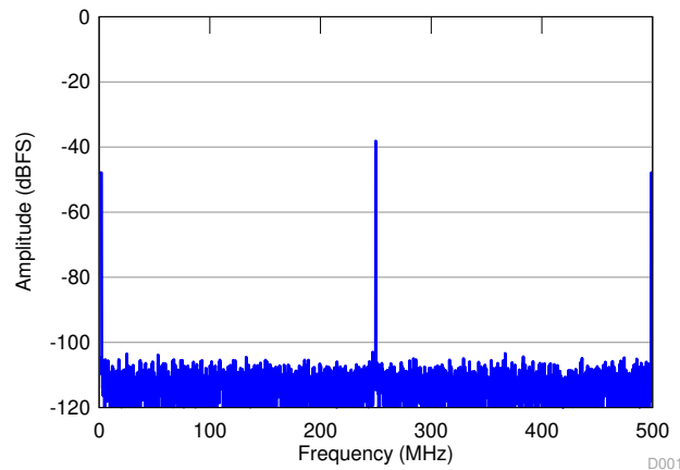
图 9-4. FFT After Bypassing the DC Offset Correction Block
