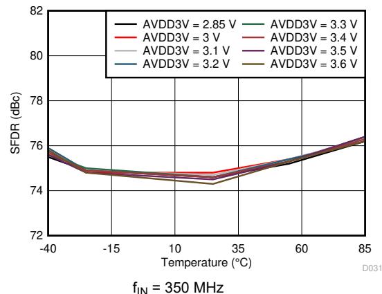
图 7-34. Spurious-Free Dynamic Range vs AVDD3V Supply and Temperature
