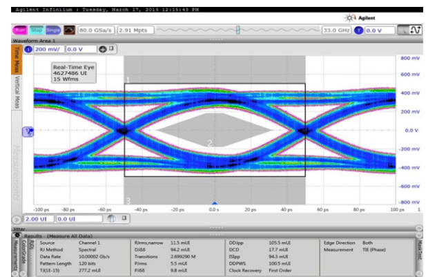
图 8-26. Eye at 10-Gbps Bit Rate with Increased Output Swing
