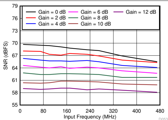
图 7-35. Signal-to-Noise Ratio vs Gain and Input Frequency
