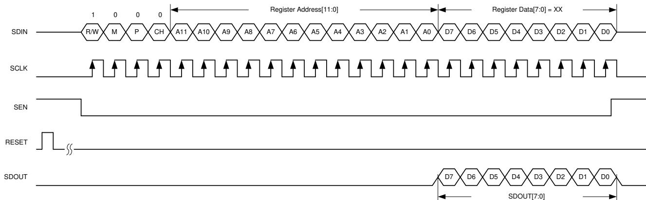
图 8-14. Serial Register Read Timing Diagram
