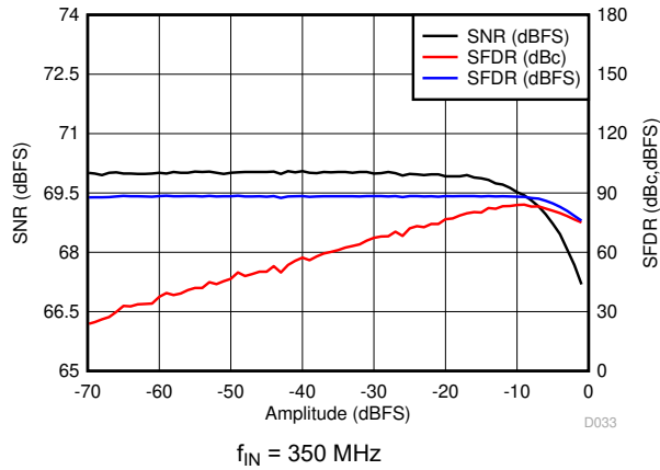
图 7-39. Performance vs Input Amplitude
