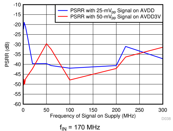
图 7-44. Power-Supply Rejection Ratio vs Test Signal Frequency
