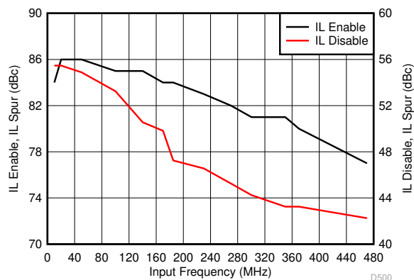
图 9-10. Typical raw IL Performance
