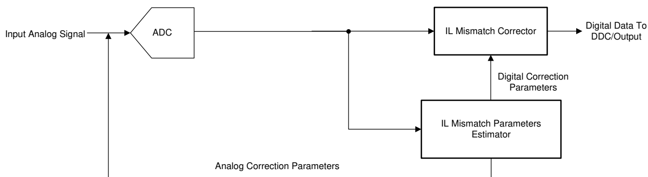
图 9-9. Block diagram of Interleaving mismatch Compensation
