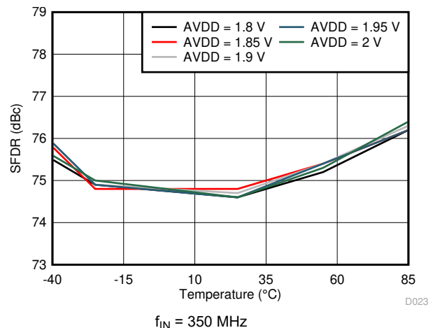
图 7-26. Spurious-Free Dynamic Range vs AVDD Supply and Temperature
