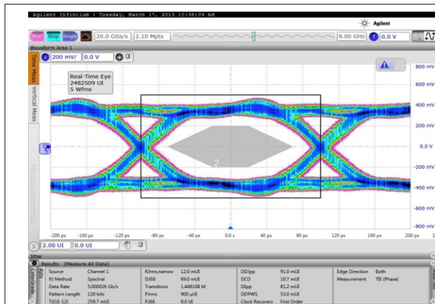
图 8-23. Eye at 5-Gbps Bit Rate with Default Output Swing
