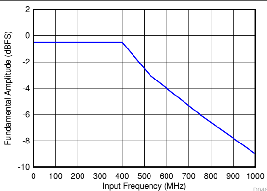
图 7-37. Maximum Supported Amplitude vs Frequency
