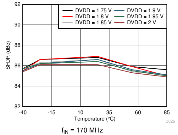
图 7-28. Spurious-Free Dynamic Range vs DVDD Supply and Temperature
