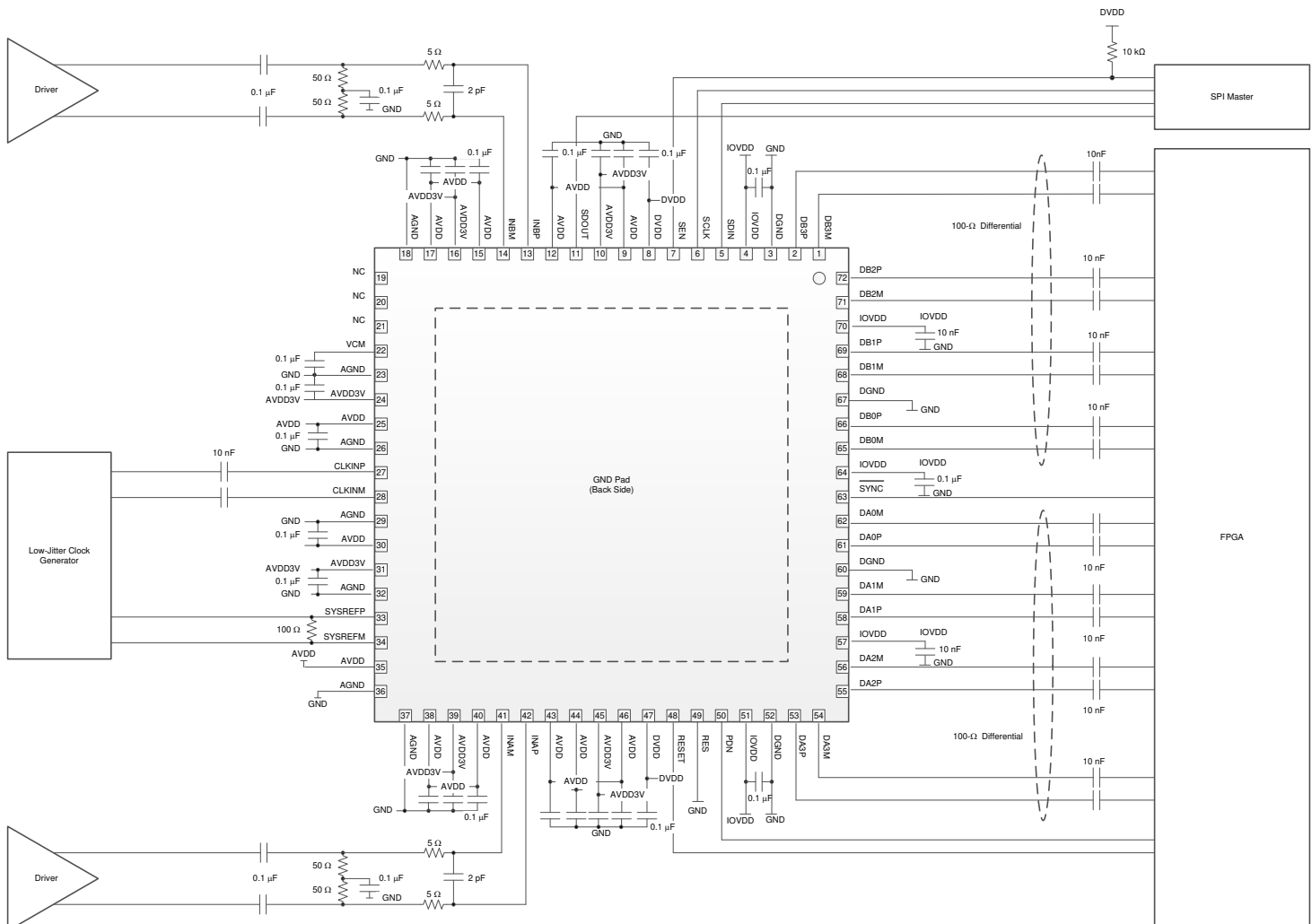
图 9-14. AC-Coupled Receiver
