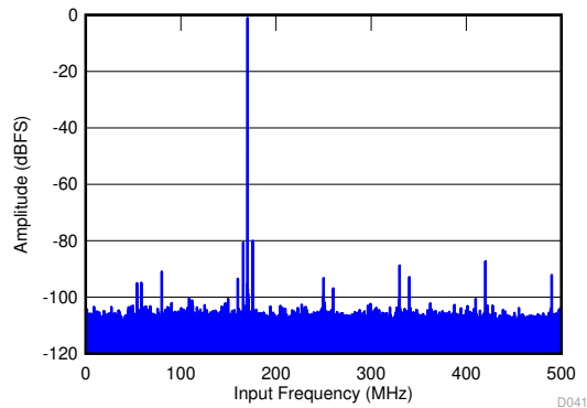
图 7-45. Power-Supply Rejection Ratio FFT for Test Signals on the AVDD Supply
