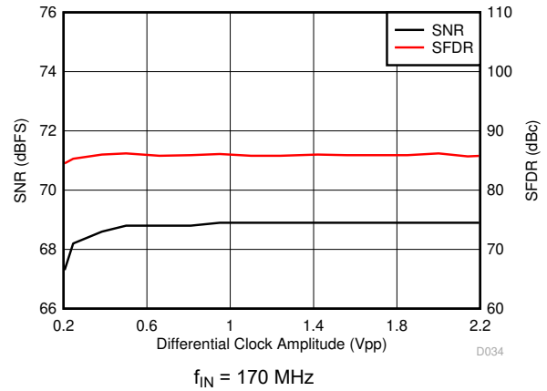
图 7-40. Performance vs Sampling Clock Amplitude
