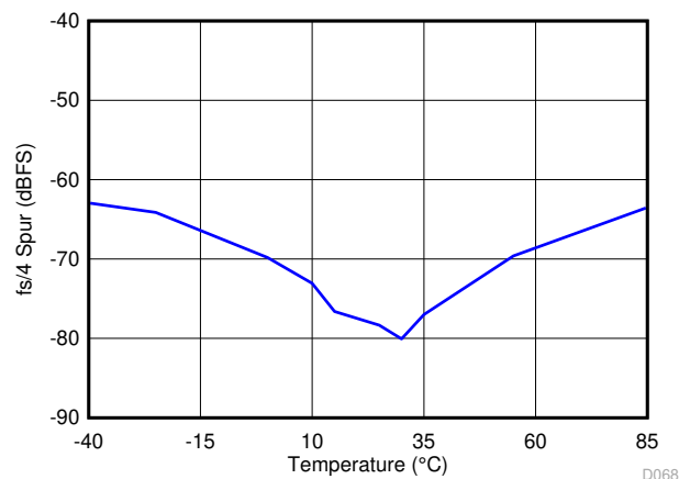
图 9-5. Variation of the f_S / 4 Spur Over Temperature
