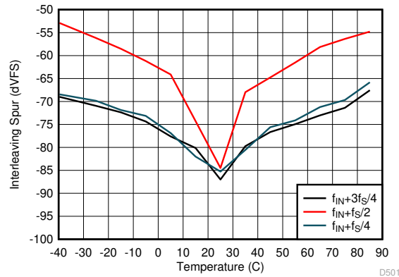
图 9-13. Residual IL Spur for signal at 400 Mhz vs Temperature after freezing IL calibration at 25°C
