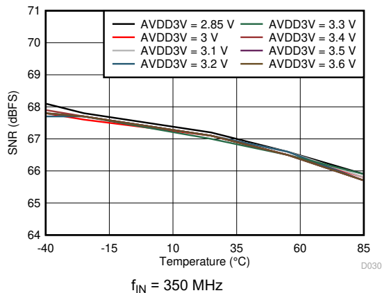
图 7-33. Signal-to-Noise Ratio vs AVDD3V Supply and Temperature
