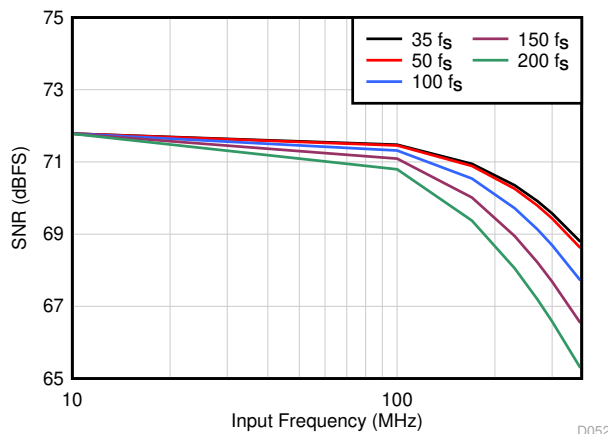
图 9-2. SNR versus Input Frequency and External Clock Jitter
