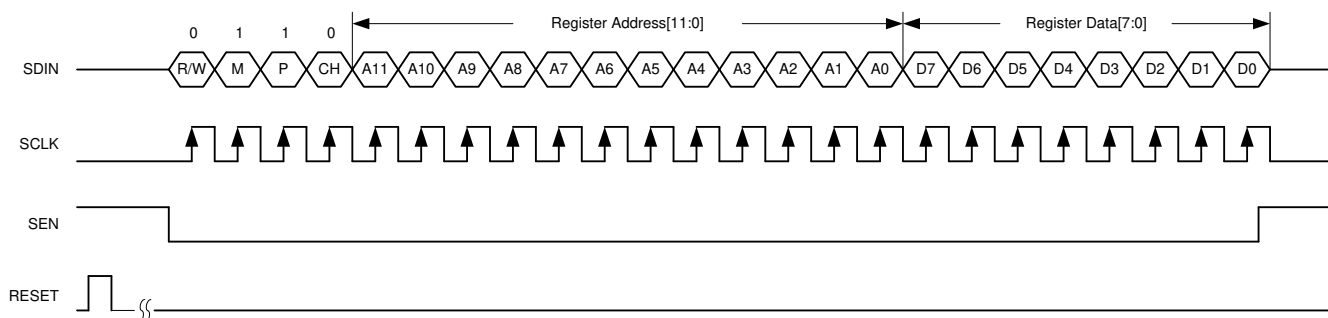
图 8-16. JESD Serial Register Write Timing Diagram
