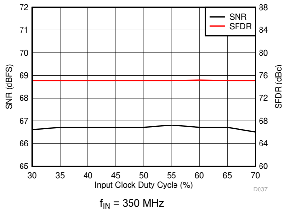
图 7-43. Performance vs Input Clock Duty Cycle
