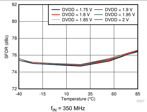
图 7-30. Spurious-Free Dynamic Range vs DVDD Supply and Temperature
