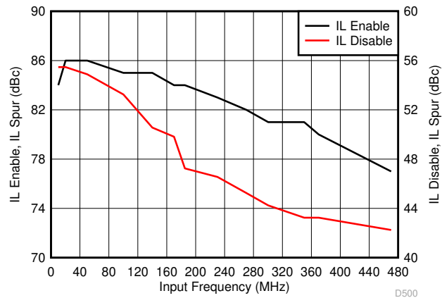
图 7-21. IL Spur vs Input Frequency
