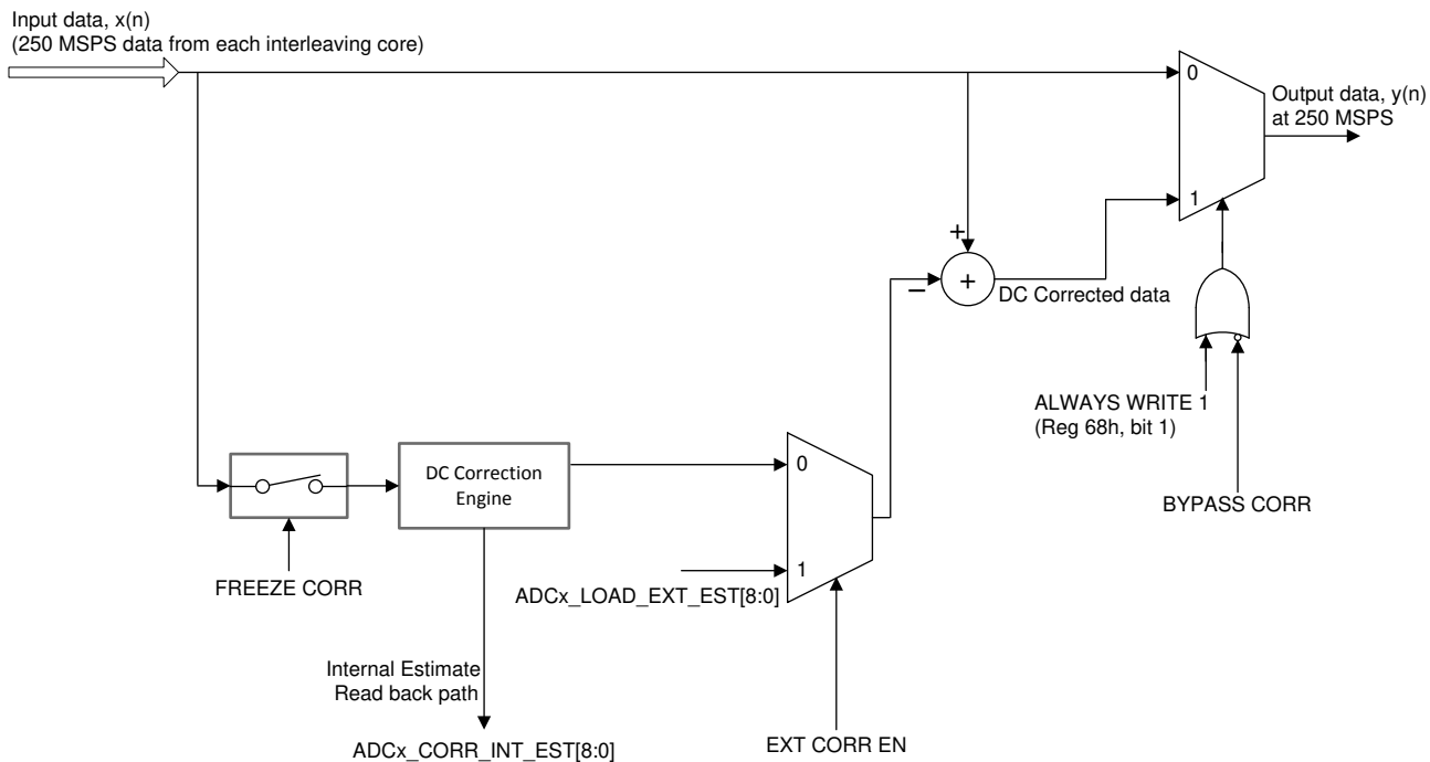
图 9-3. DC Offset Correction Block Diagram
