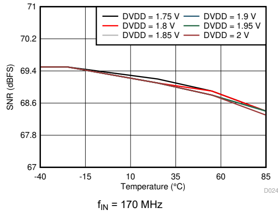
图 7-27. Signal-to-Noise Ratio vs DVDD Supply and Temperature
