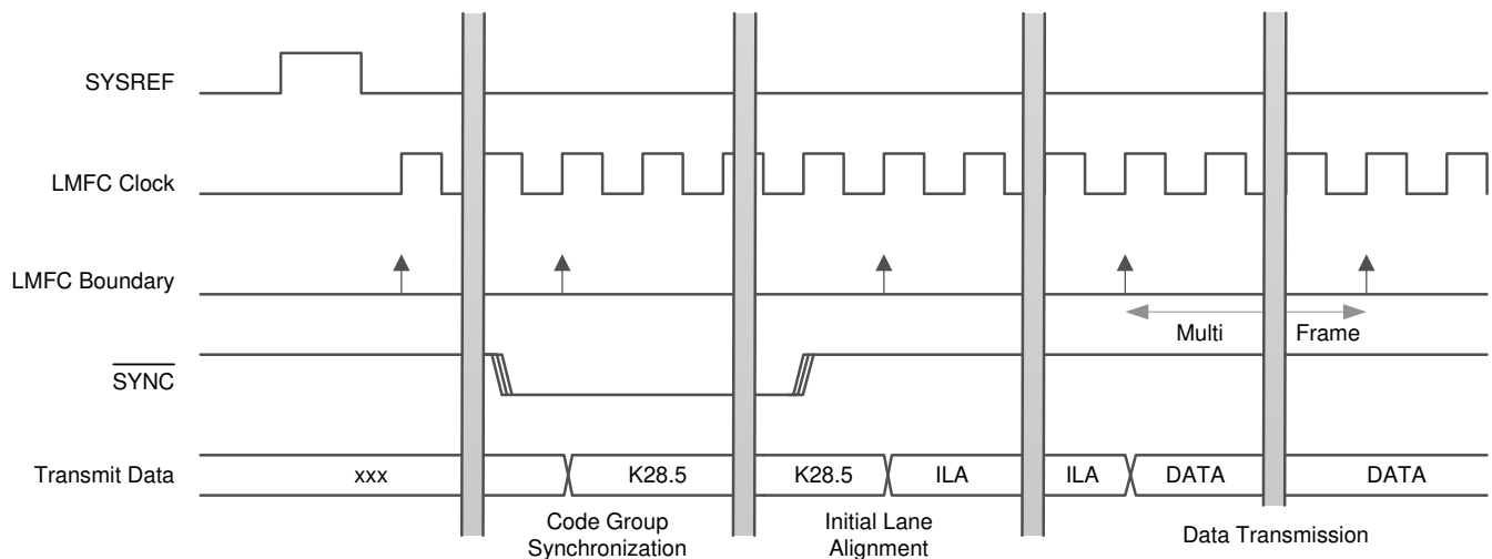
图 8-21. Lane Alignment Sequence
