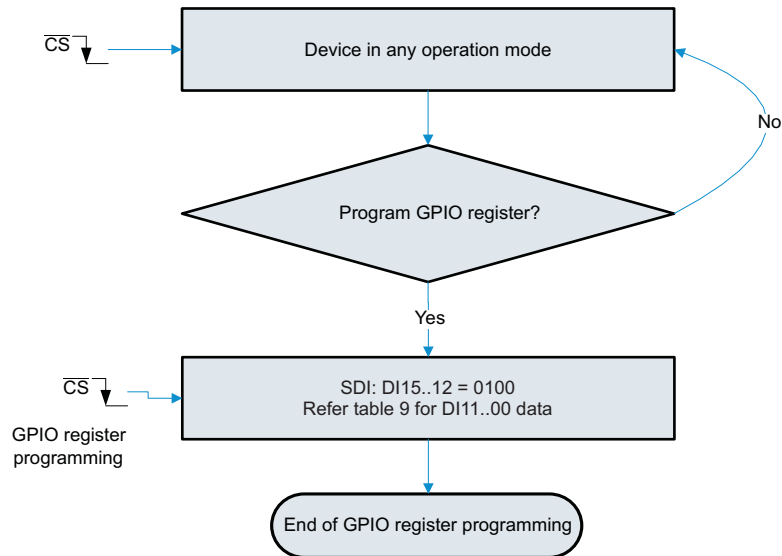
Figure 16. GPIO Program Register Programming Flowchart
