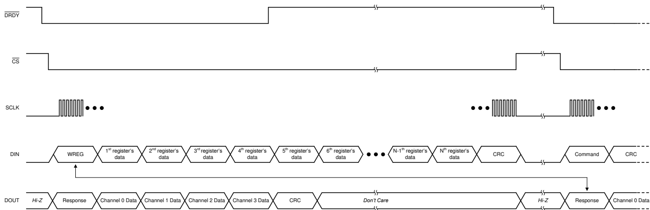
图 8-19. Writing Registers
