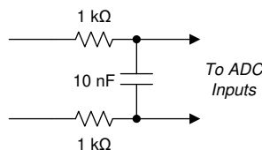
图 9-1. Recommended Antialias Filter
