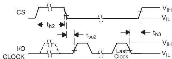
Figure 27. \overline{CS} and I/O CLOCK Voltage Waveforms
