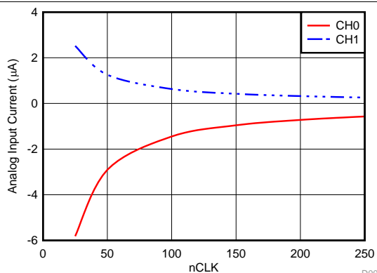
图 30. Analog Input Current in Autonomous modes with nCLK
