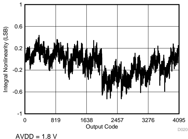
图 20. Typical INL in Manual Mode
