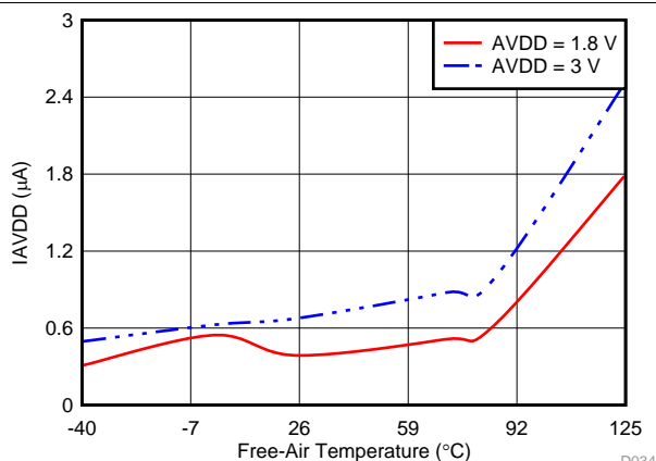
图 30. Analog Input Current in Autonomous modes with nCLK
