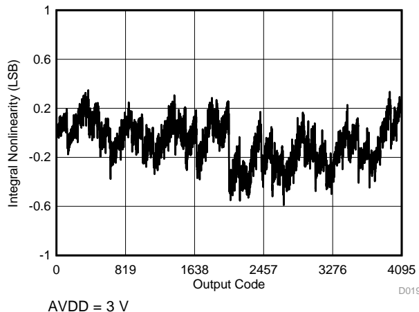
图 19. Typical INL in Manual Mode
