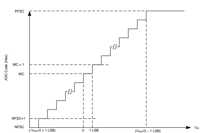
图 44. Ideal Transfer Characteristics for Pseudo-Differential Configuration
