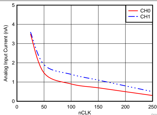
图 31. Analog Input Current in Autonomous modes with nCLK
