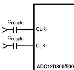
Figure 6-8. Differential Input Clock Connection
