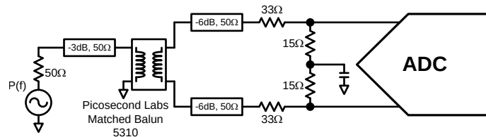
图 64. 50-Ω Source, Bandwidth Measurement Network
