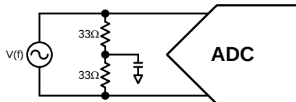
图 65. Low-Ω Source Bandwidth Measurement (Simplified)
