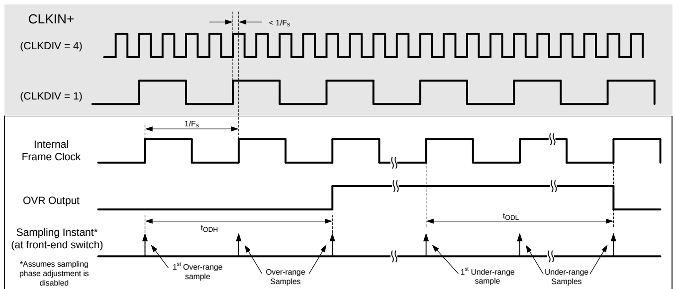
图 2. Overage (OVR) Timing Diagram
