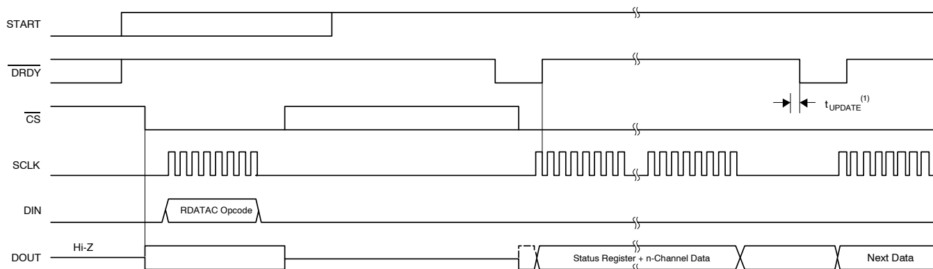
Figure 37. RDATAC Usage
