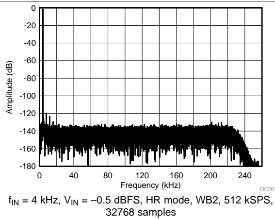
Figure 6. Output Spectrum
