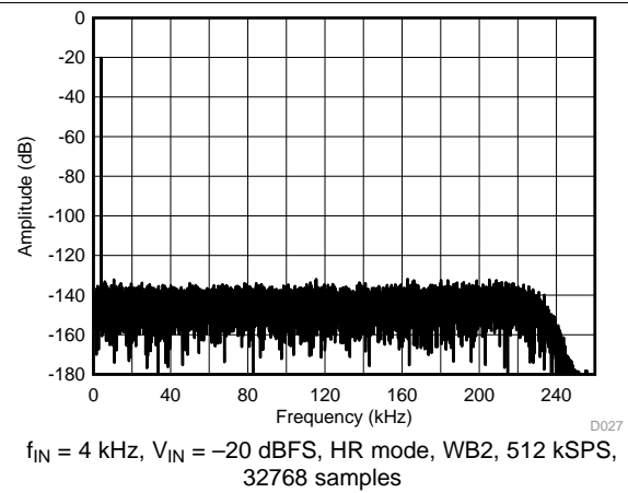
Figure 7. Output Spectrum
